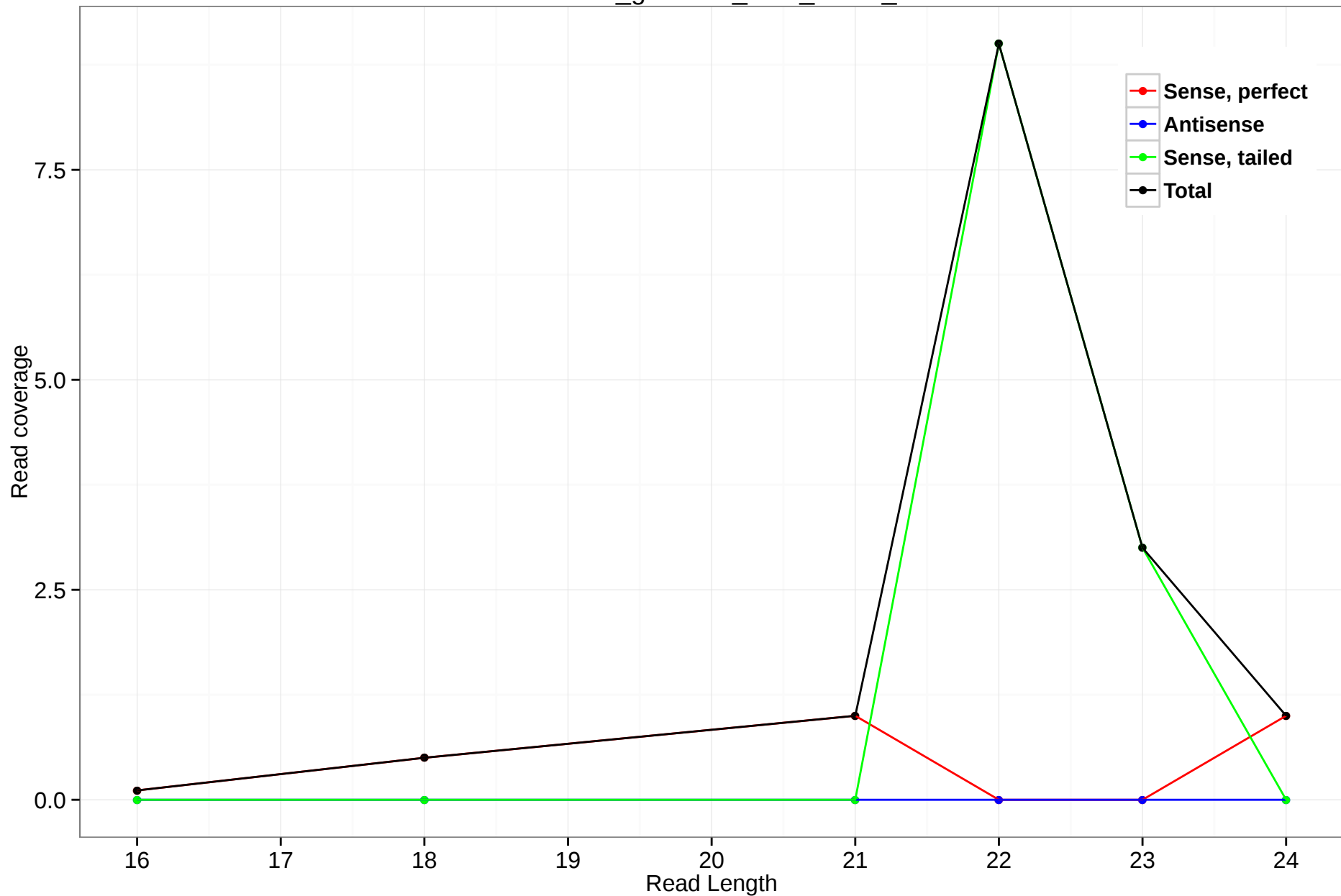
rheMac3_genscan_chr8_165.7_4
