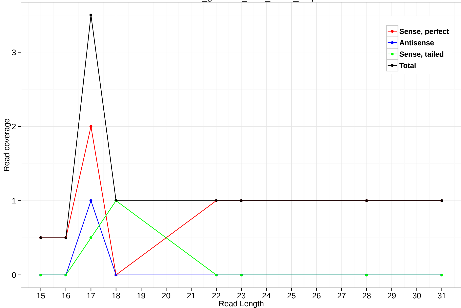
rheMac3_genscan_chr8_165.6_7.5p
