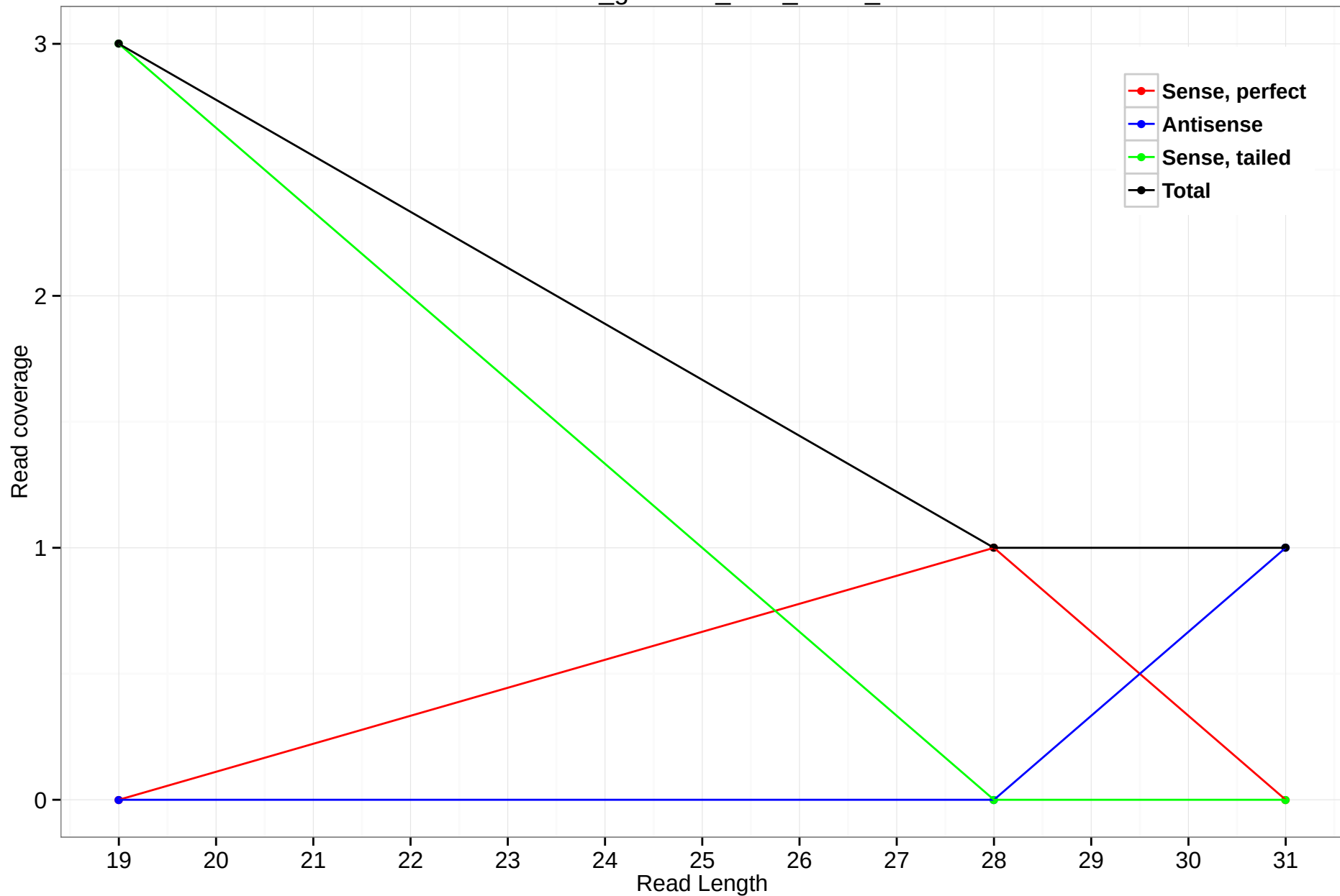
rheMac3_genscan_chr8_165.2_20
