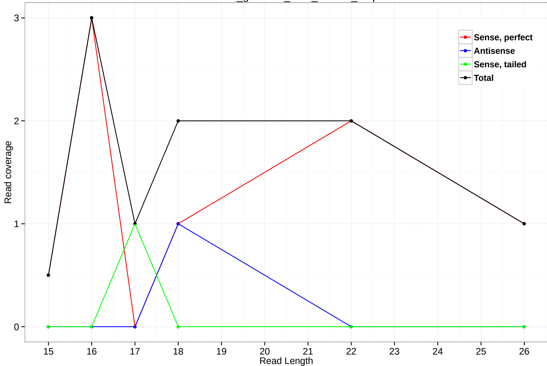
rheMac3_genscan_chr8_165.23_4.5p
