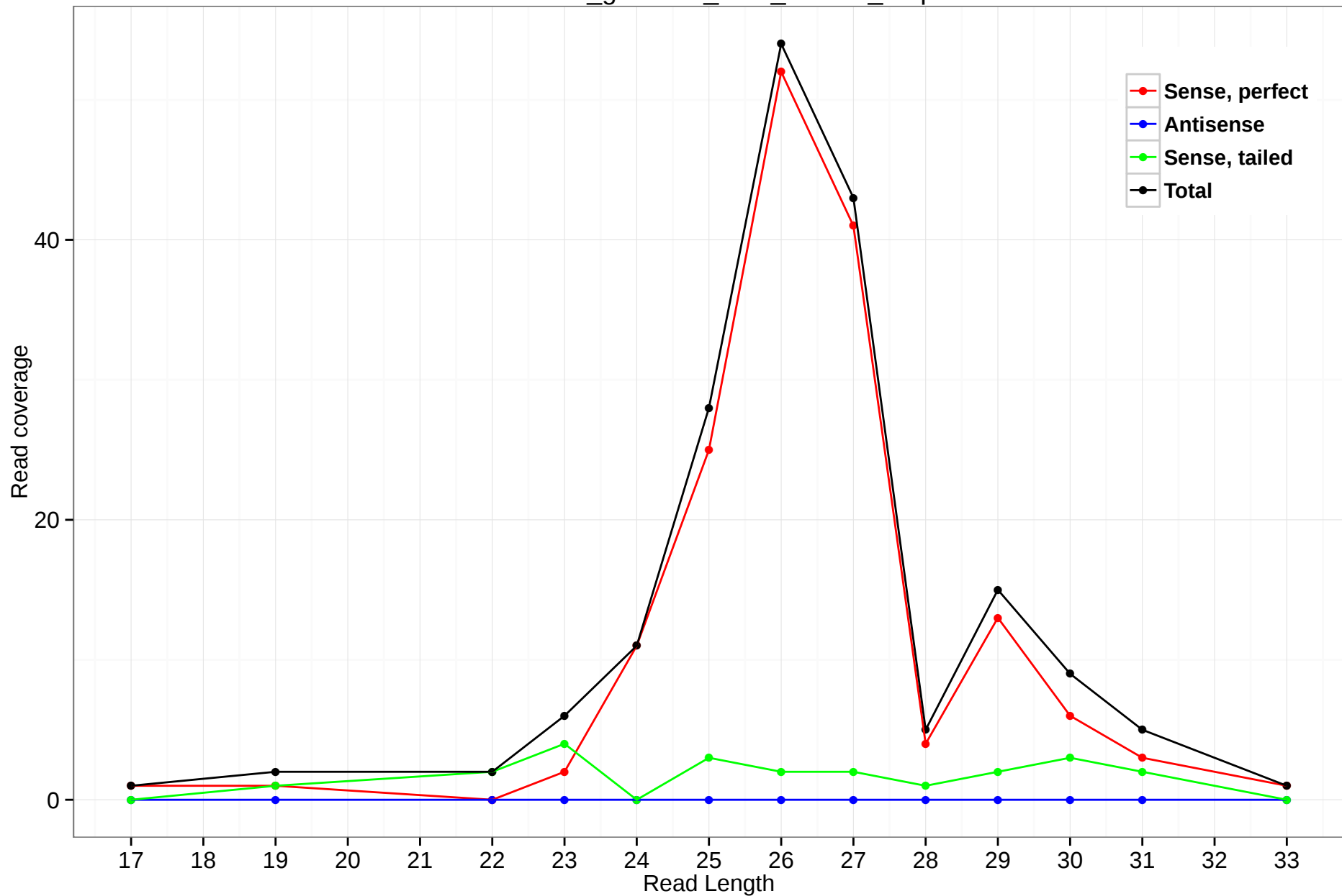
rheMac3_genscan_chr8_165.12_9.5p
