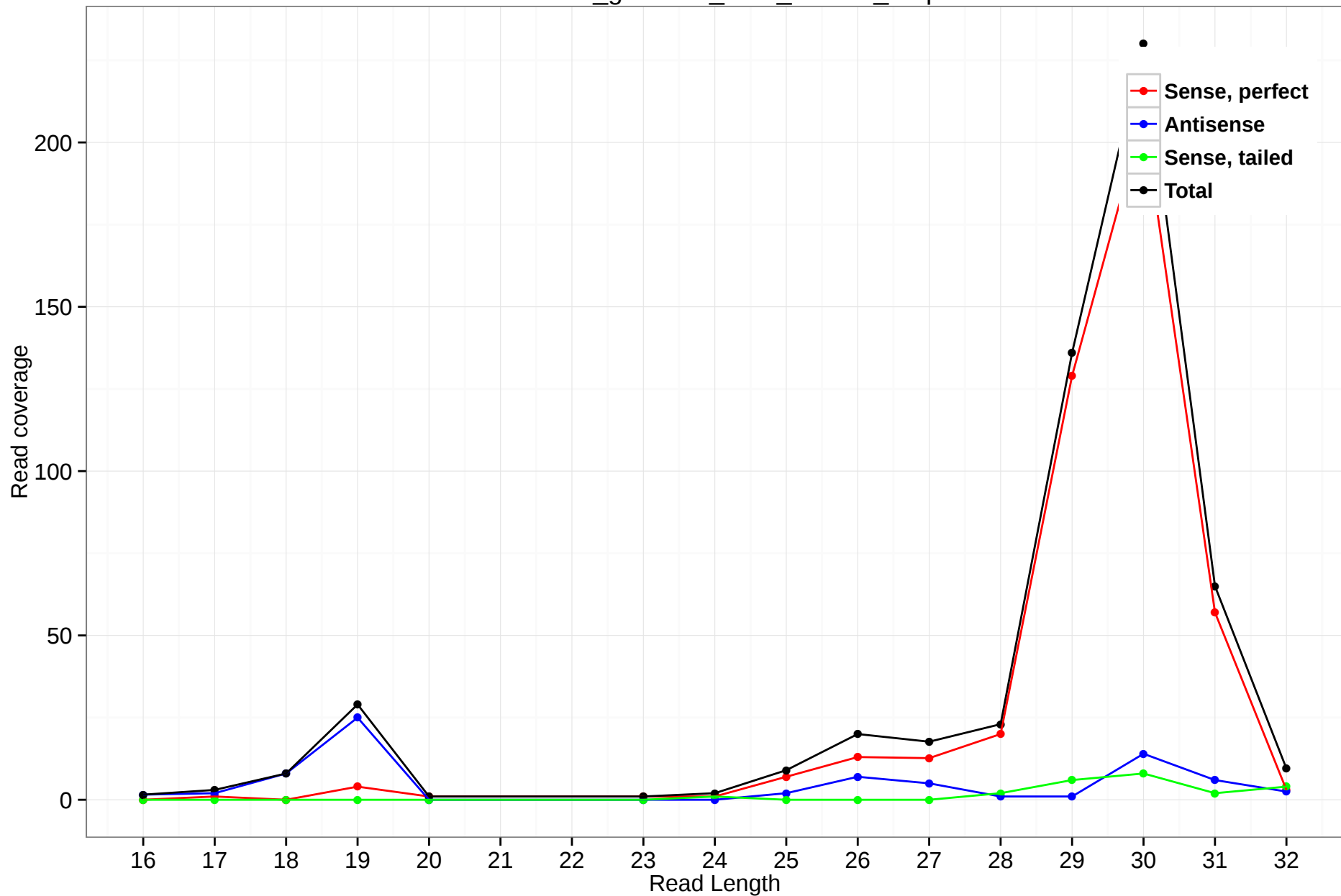
rheMac3_genscan_chr8_165.12_9.3p
