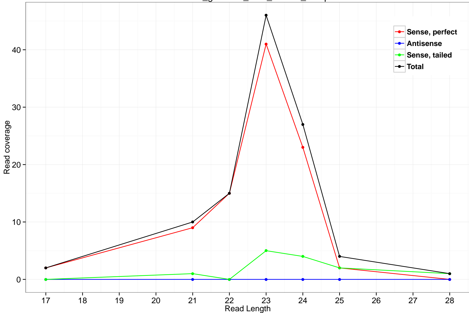
rheMac3_genscan_chr8_163.38_23.3p
