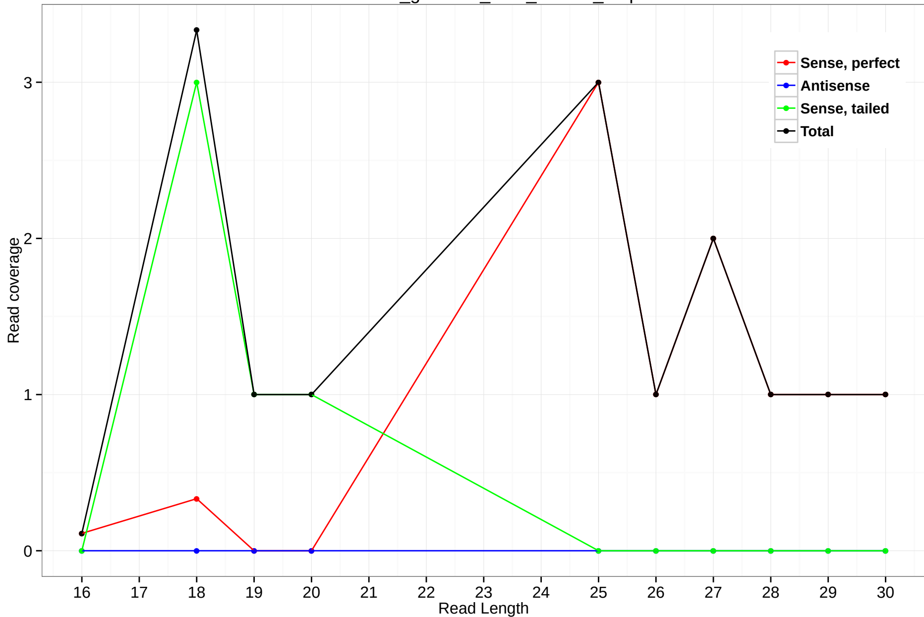
rheMac3_genscan_chr8_163.35_6.3p
