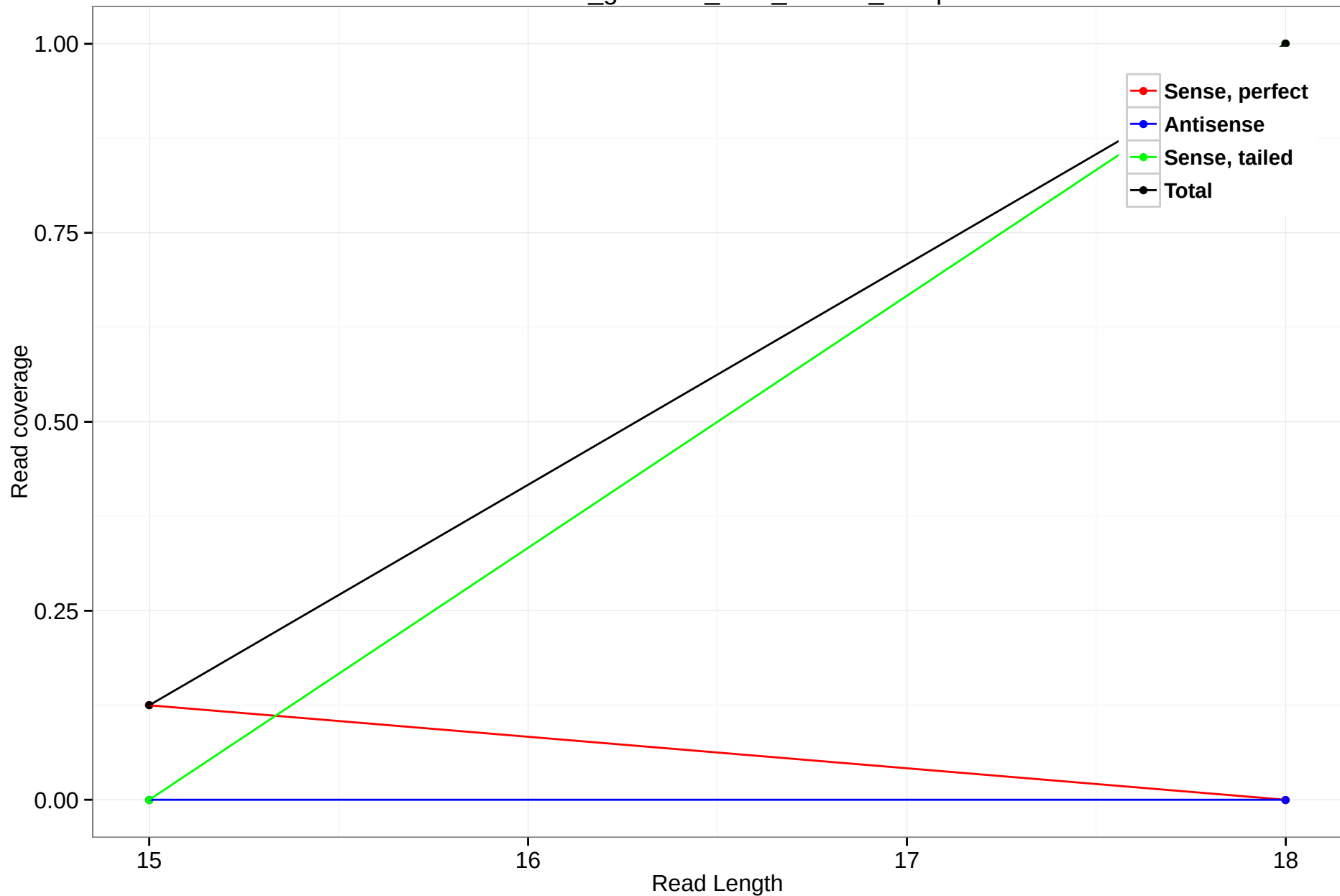
rheMac3_genscan_chr8_163.24_10.3p
