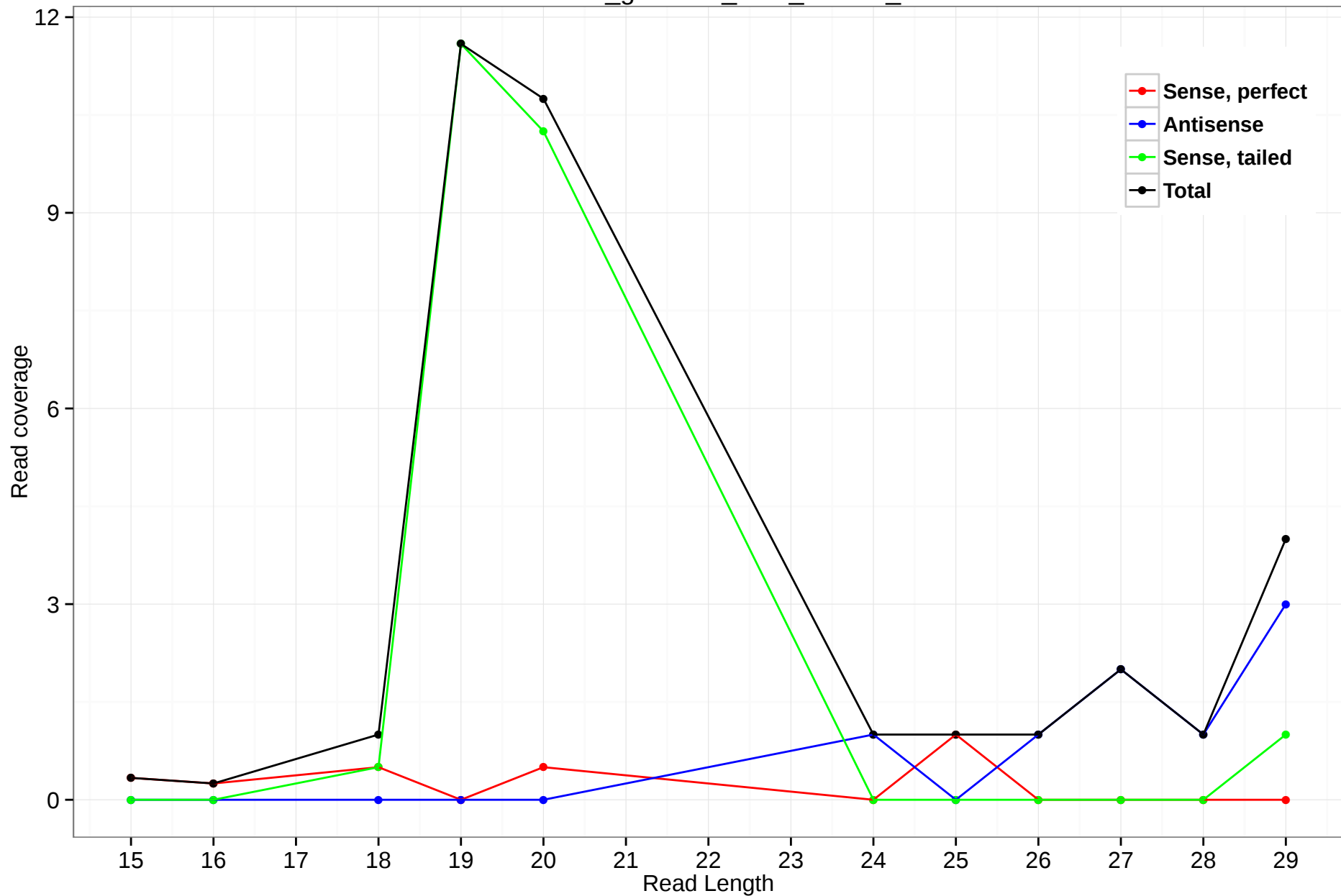
rheMac3_genscan_chr8_163.22_6
