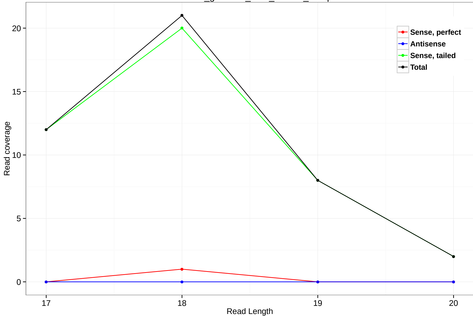
rheMac3_genscan_chr8_162.20_20.5p
