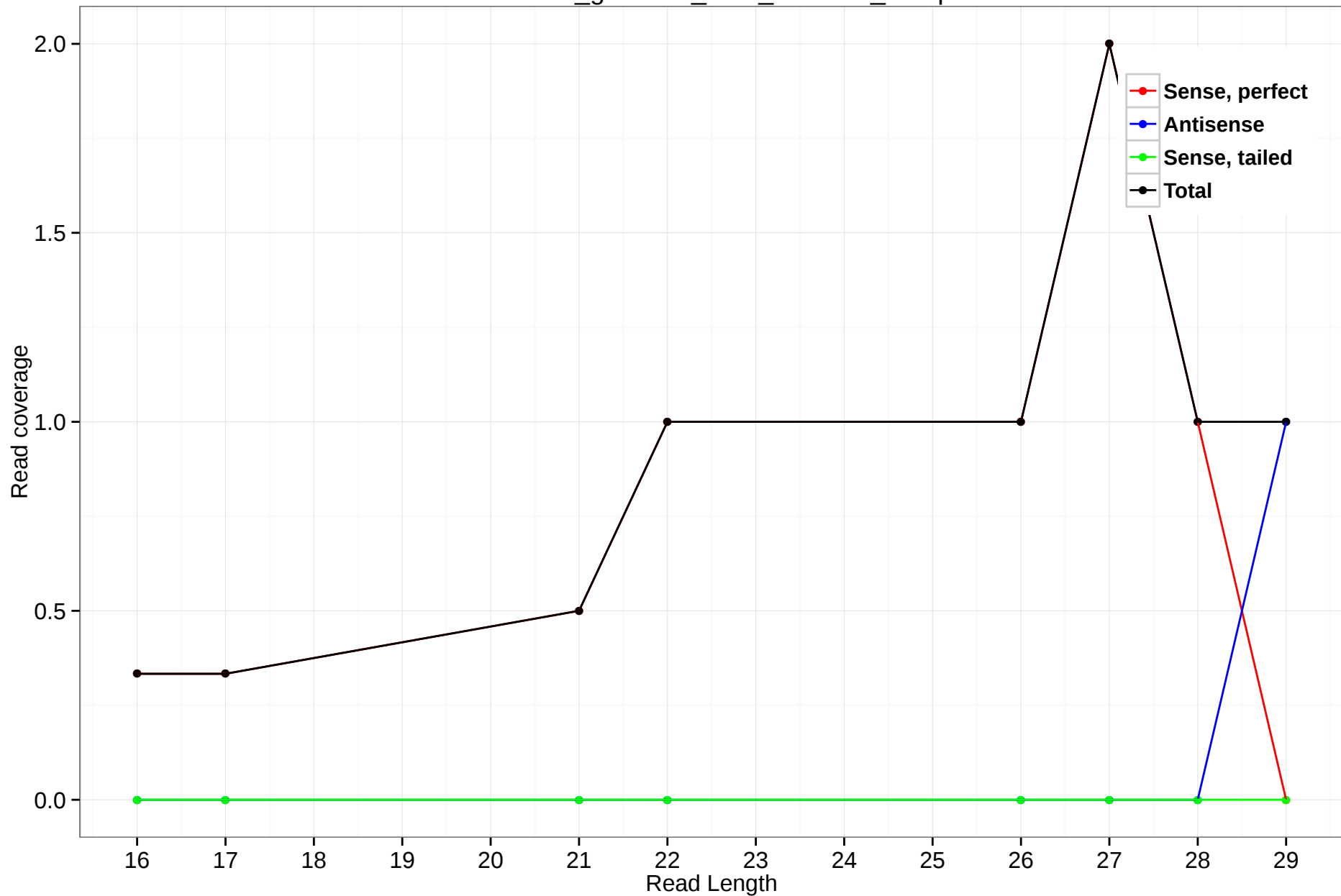
rheMac3_genscan_chr8_160.144_24.3p
