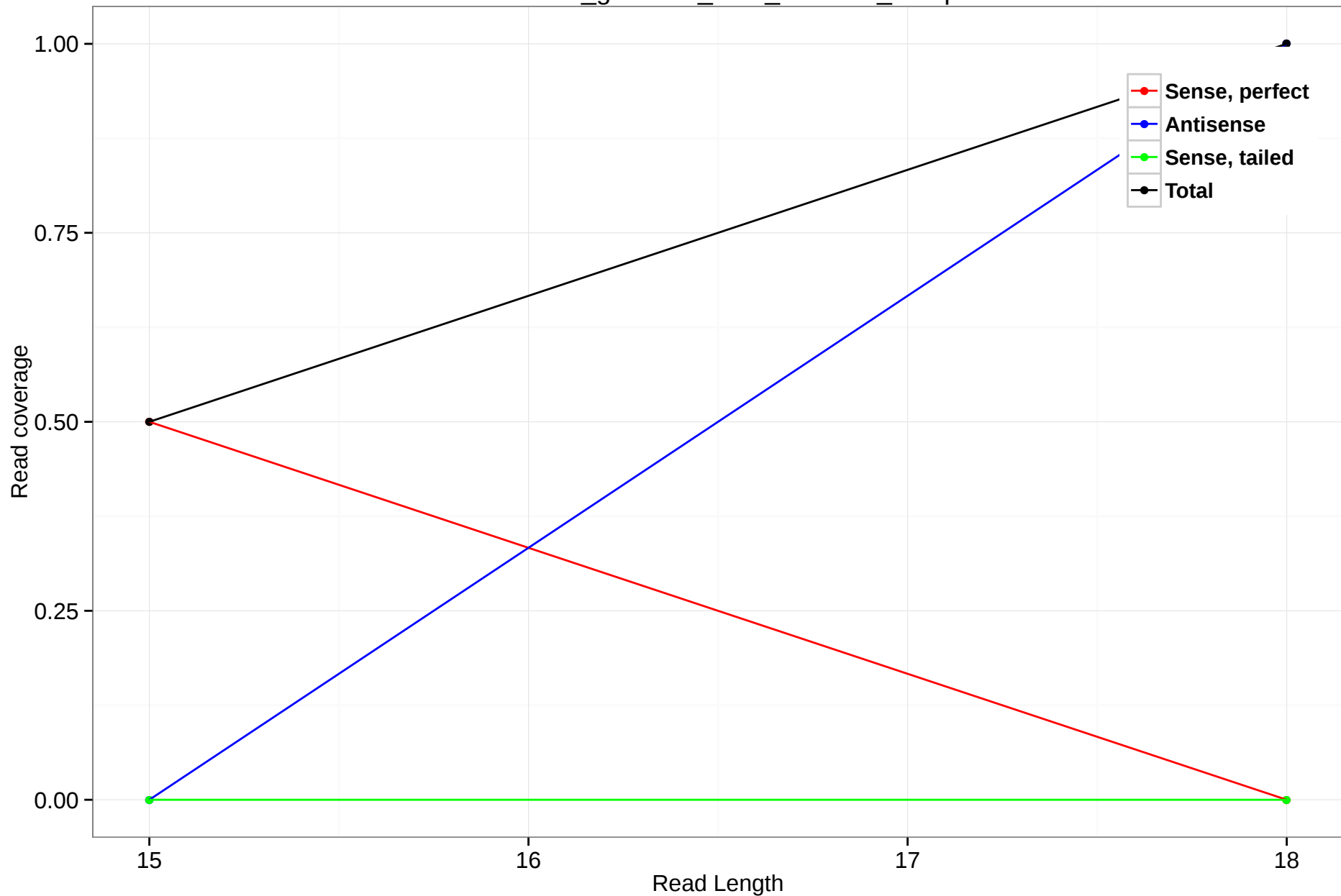
rheMac3_genscan_chr8_160.144_10.3p
