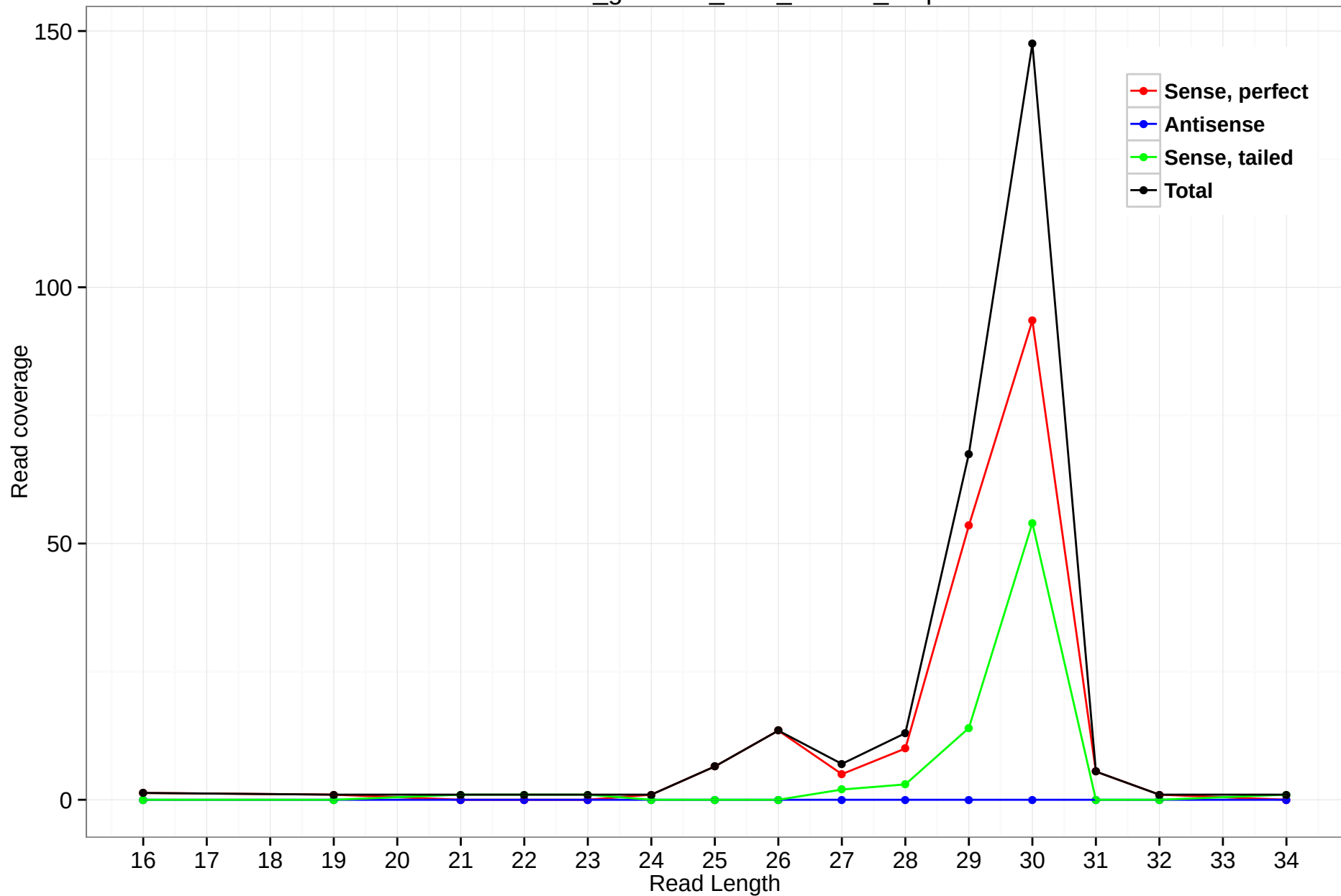
rheMac3_genscan_chr8_155.84_1.3p
