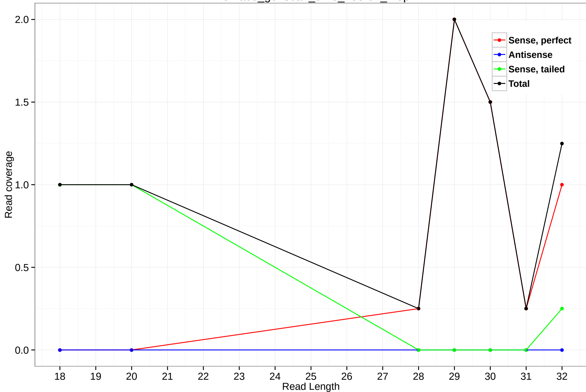
rheMac3_genscan_chr8_155.67_1.5p
