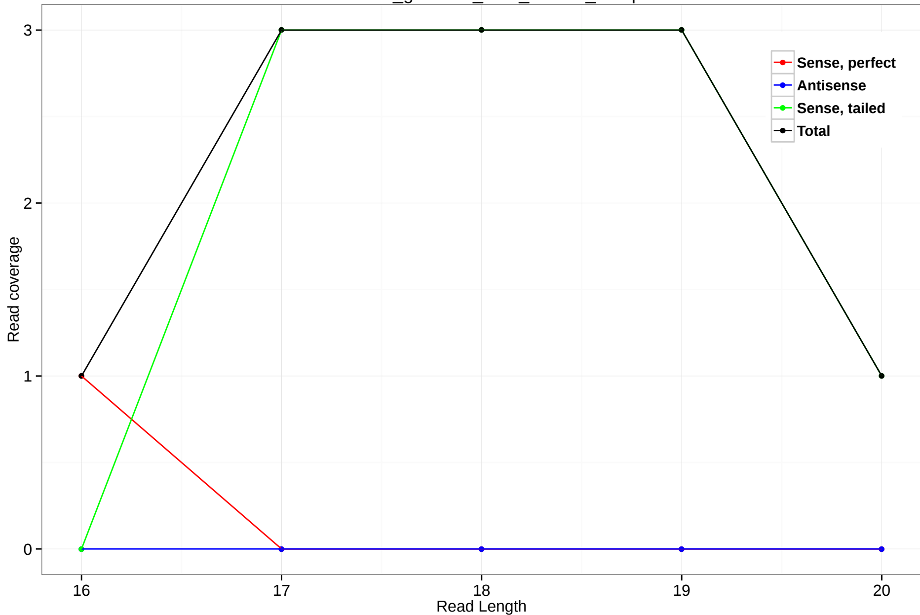
rheMac3_genscan_chr8_155.54_12.3p
