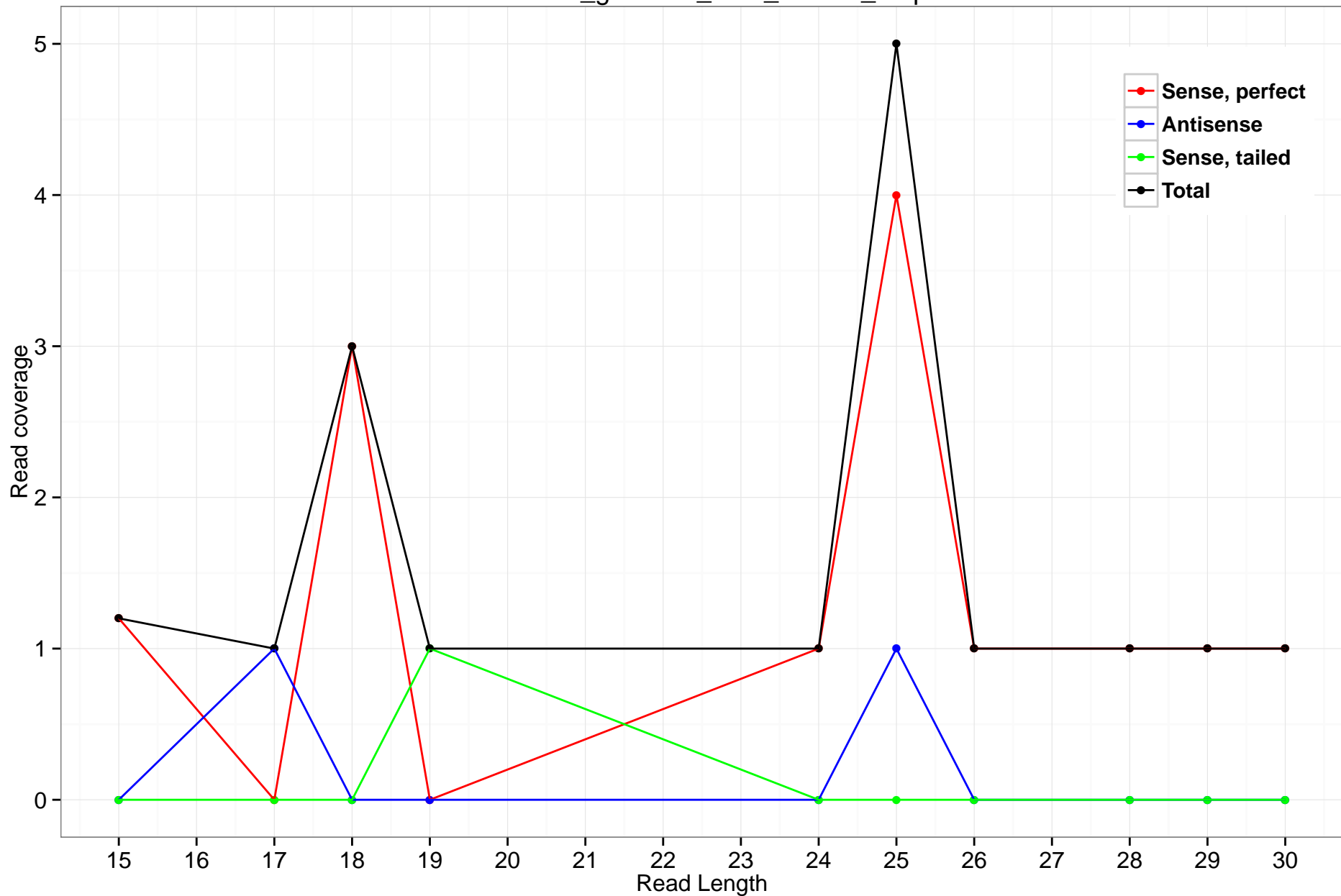
rheMac3_genscan_chr8_155.35_1.5p
