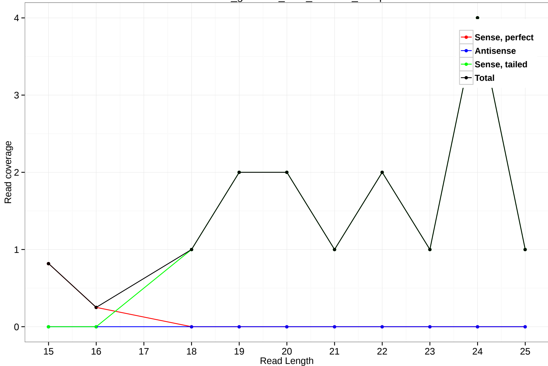
rheMac3_genscan_chr8_155.201_16.3p
