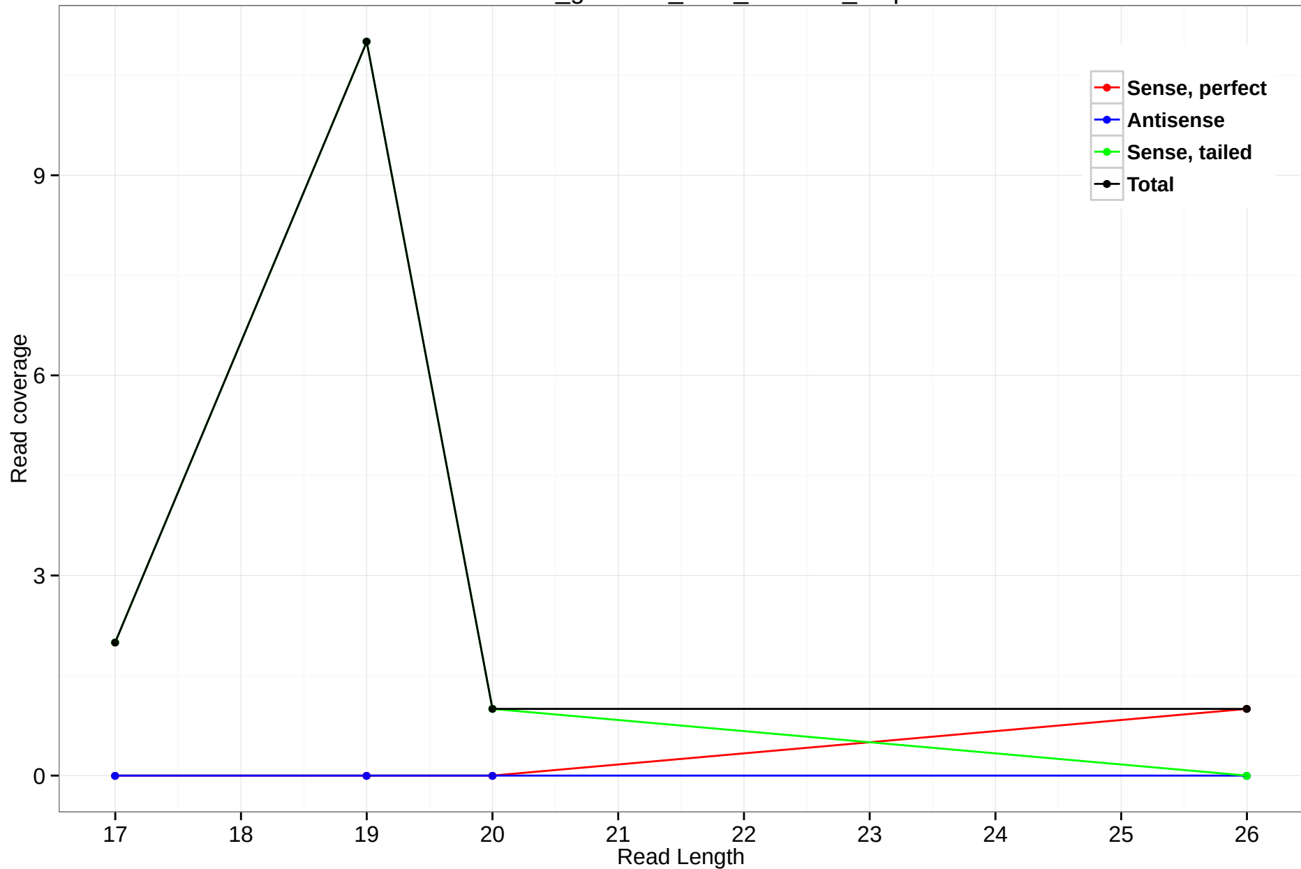
rheMac3_genscan_chr8_155.160_7.5p
