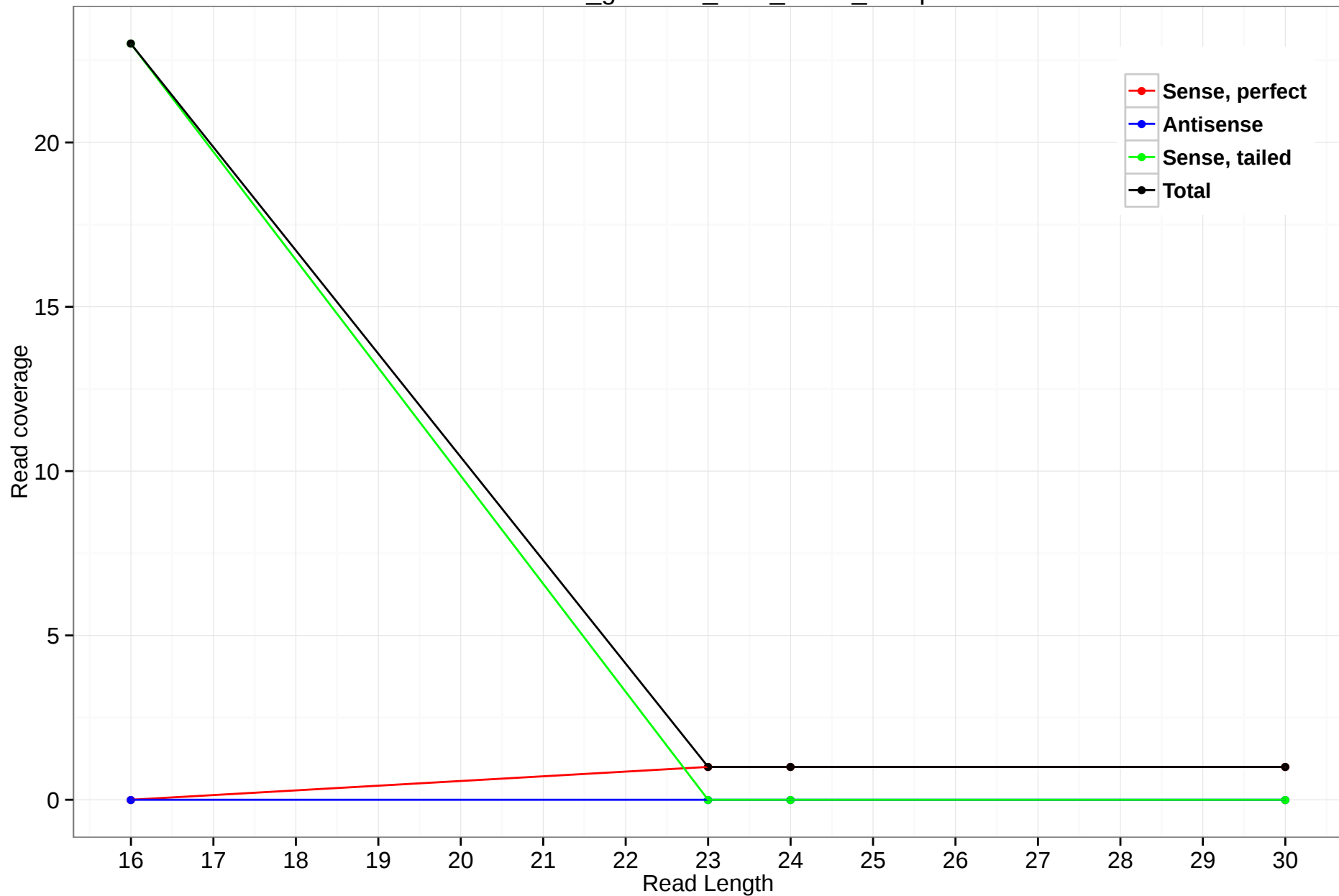
rheMac3_genscan_chr8_154.2_12.5p
