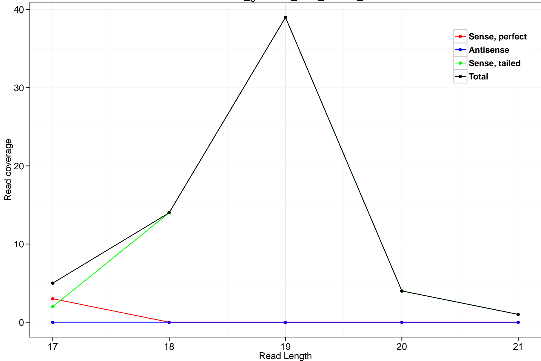
rheMac3_genscan_chr8_153.70_4
