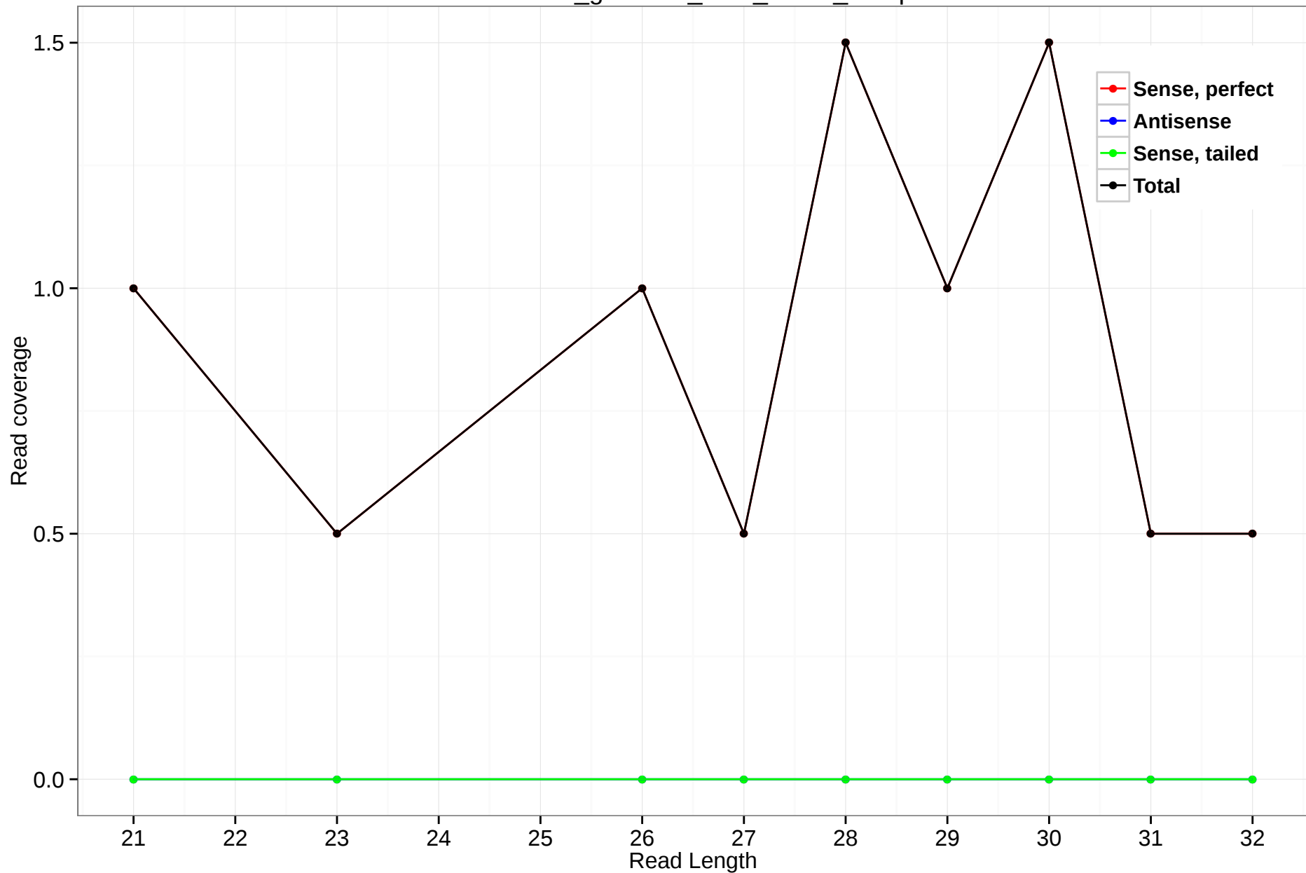
rheMac3_genscan_chr8_148.3_16.5p
