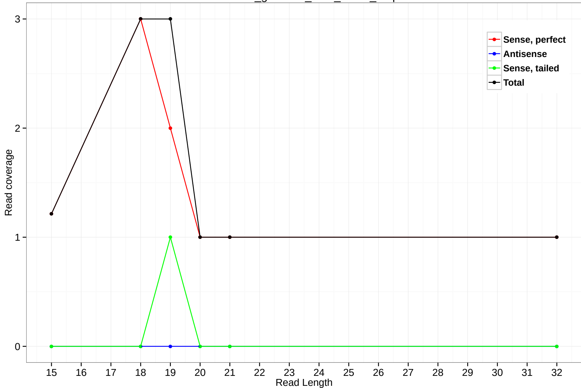
rheMac3_genscan_chr8_144.4_0.3p
