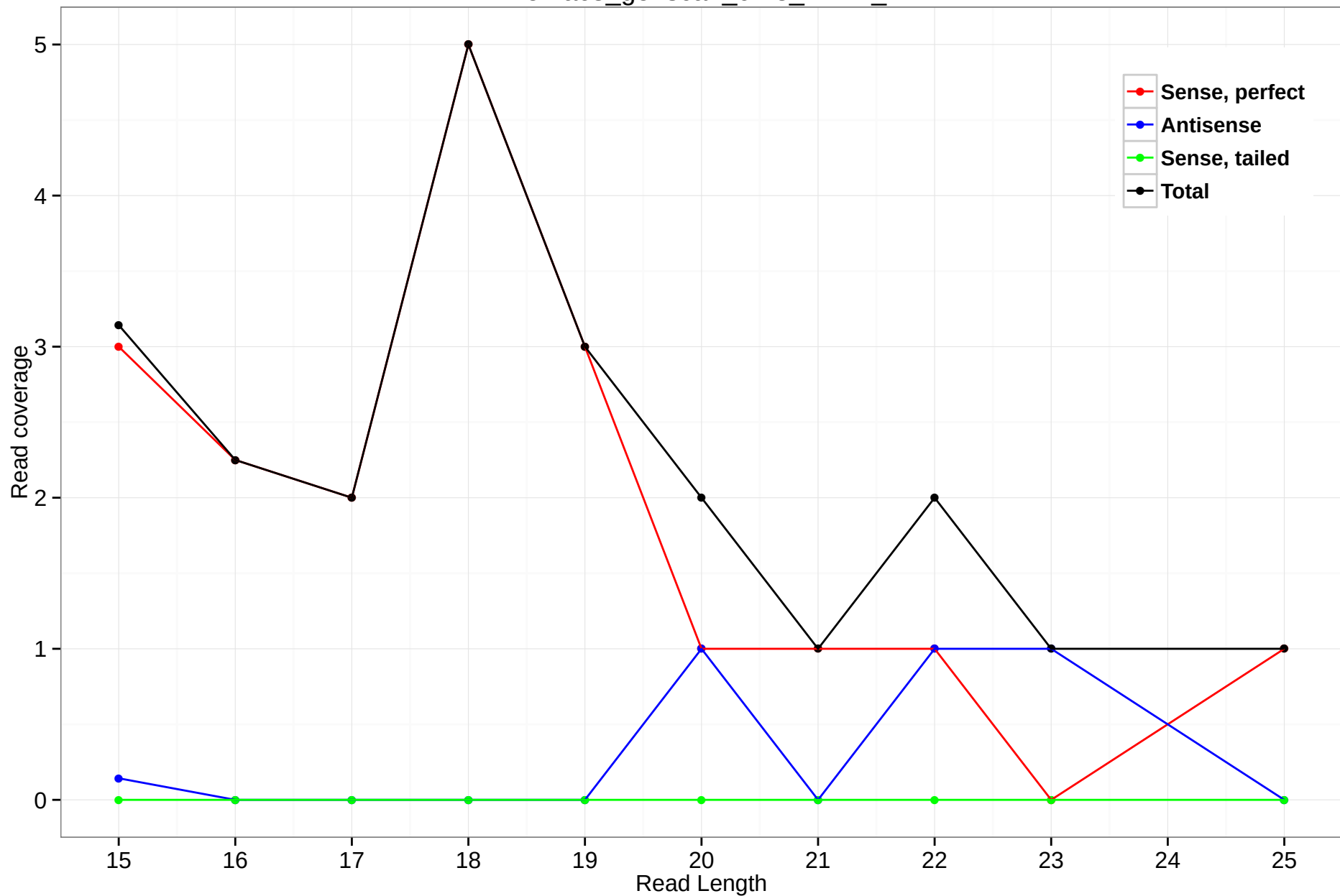
rheMac3_genscan_chr8_144.1_2
