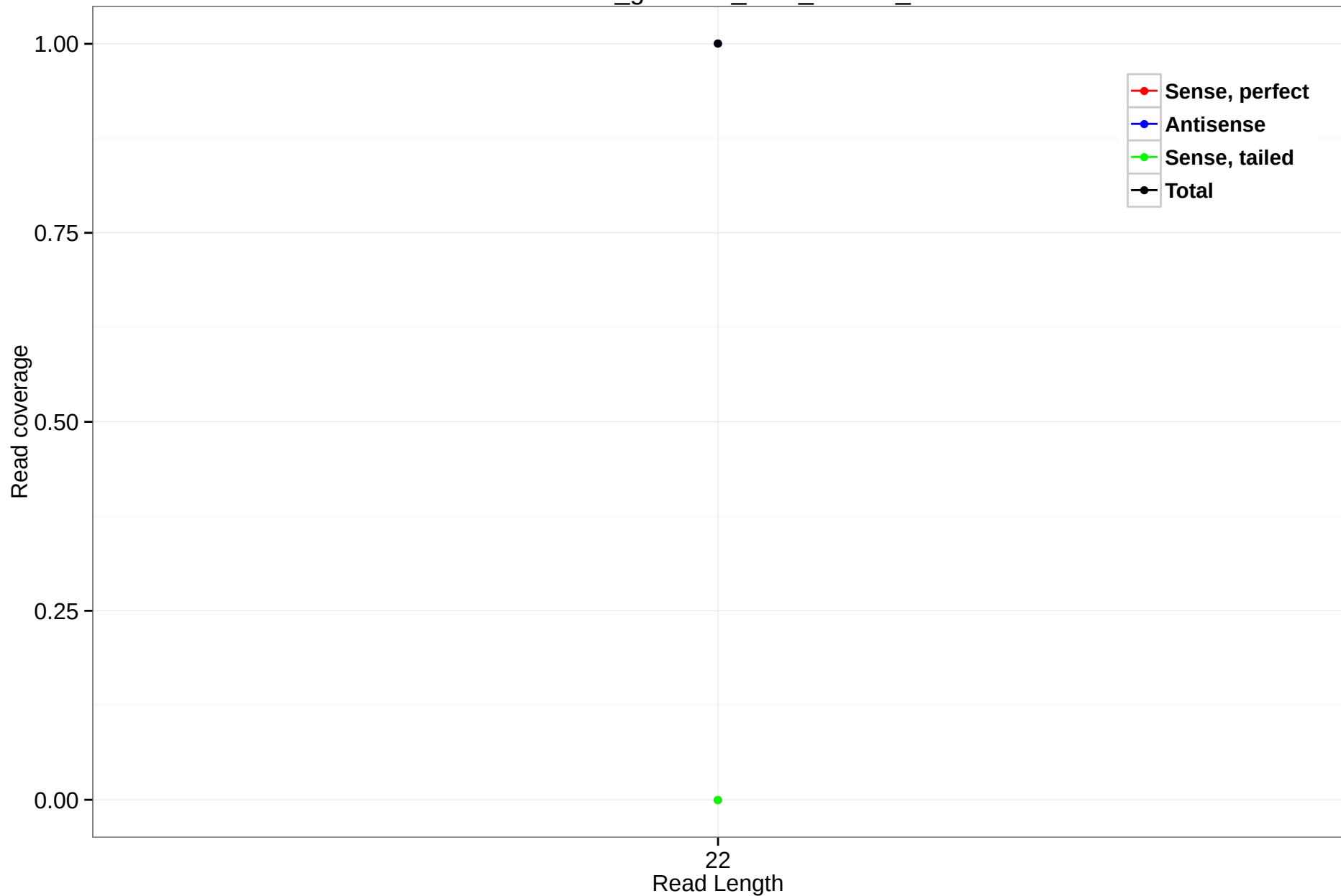
rheMac3_genscan_chr8_142.79_6
