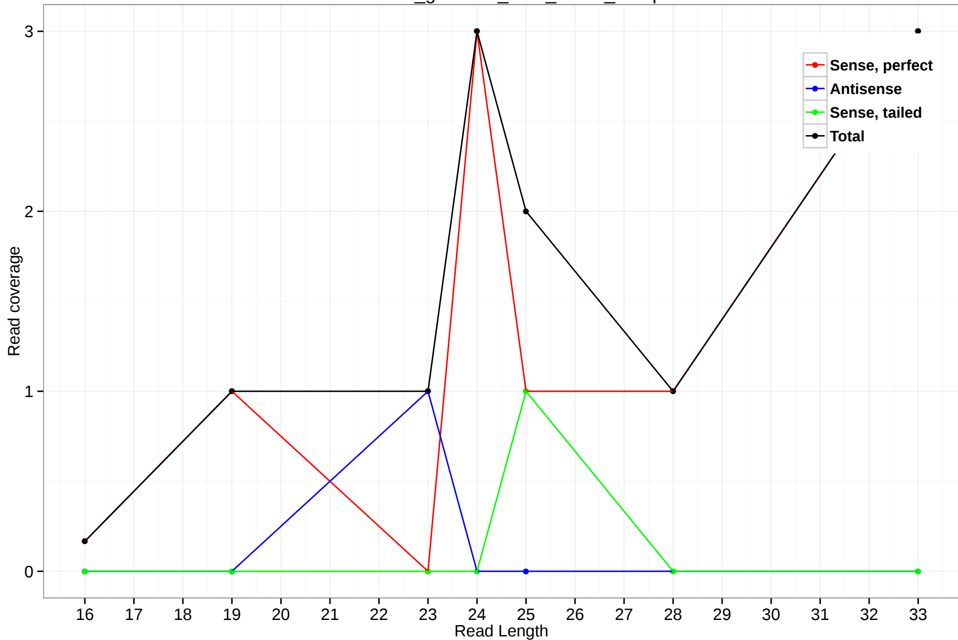
rheMac3_genscan_chr8_13.49_26.5p
