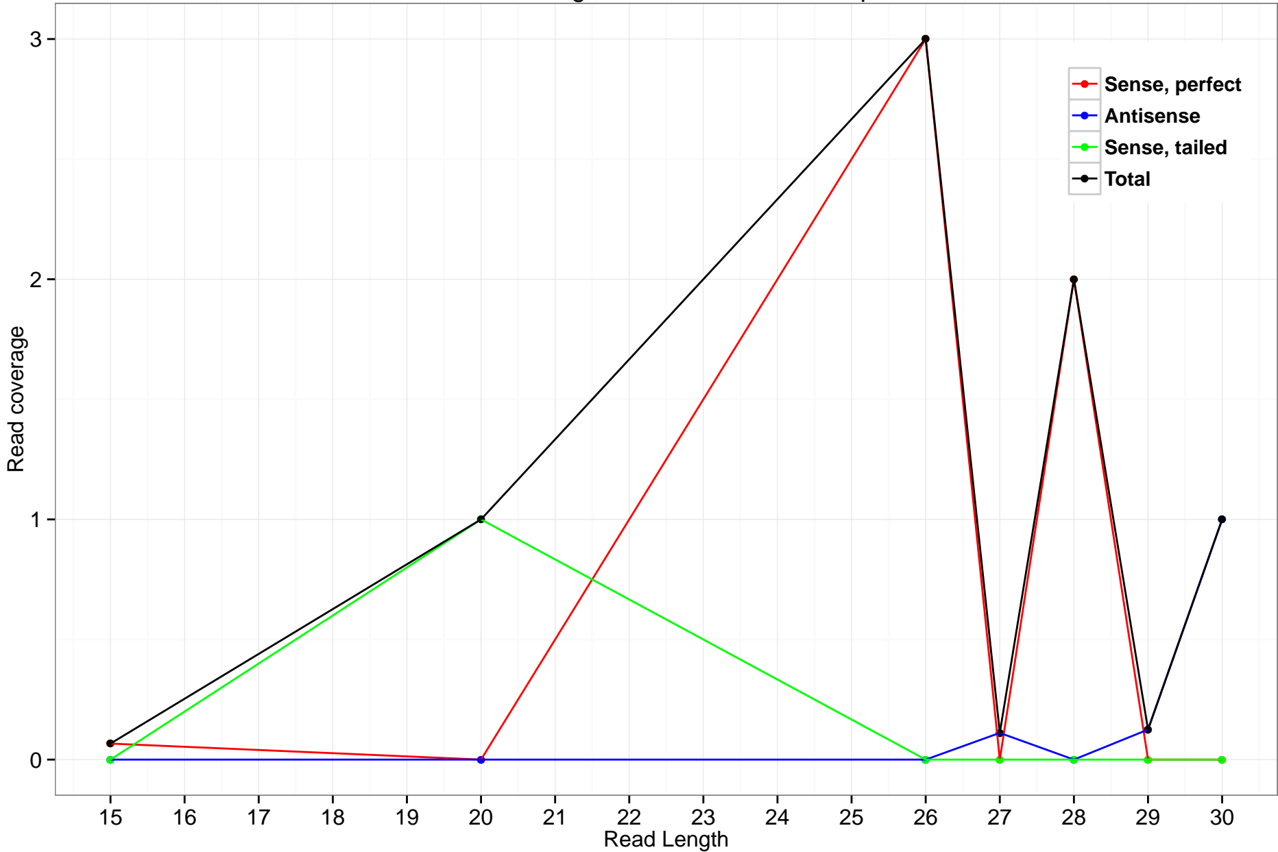
rheMac3_genscan_chr8_13.22_0.5p
