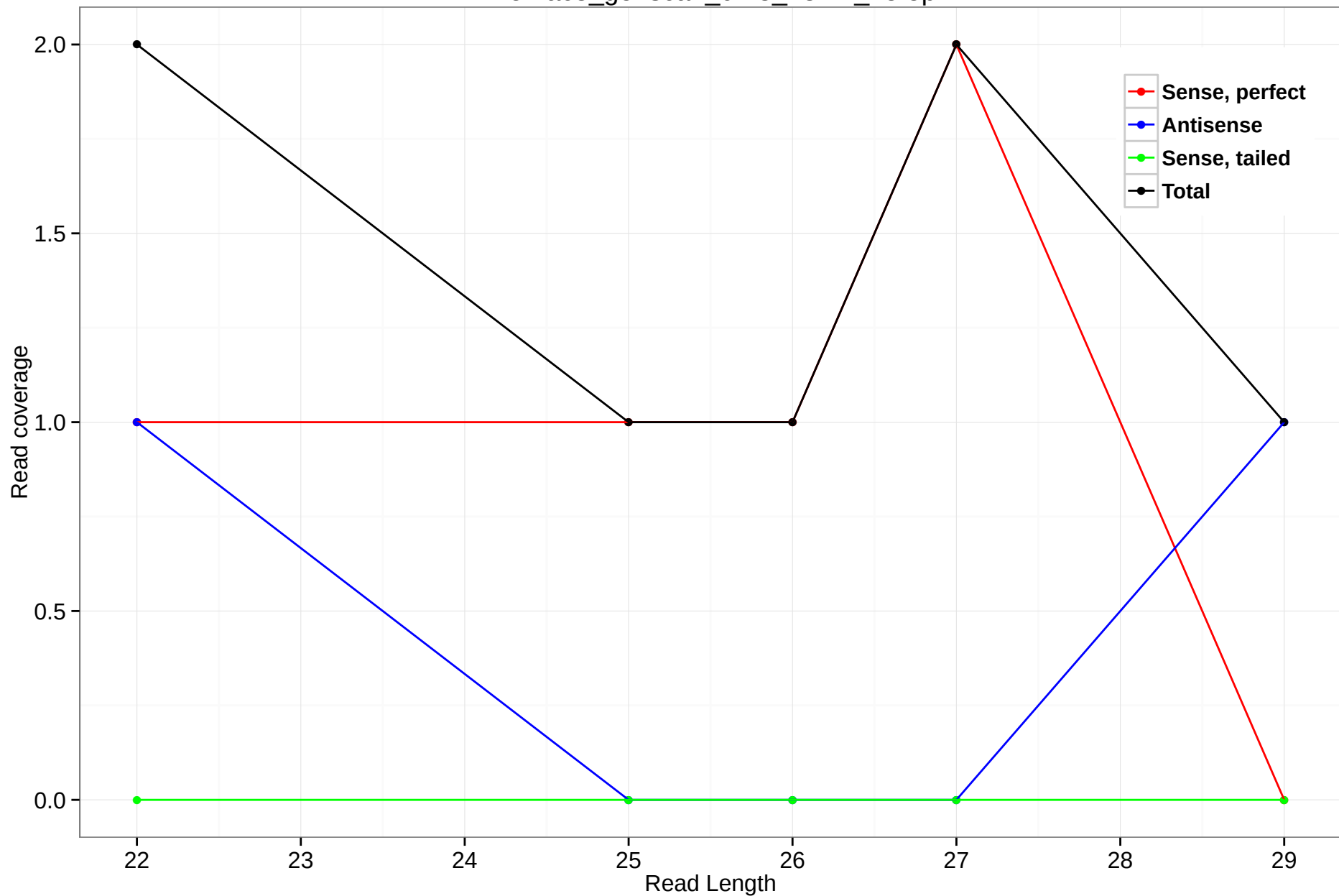
rheMac3_genscan_chr8_13.12_15.5p
