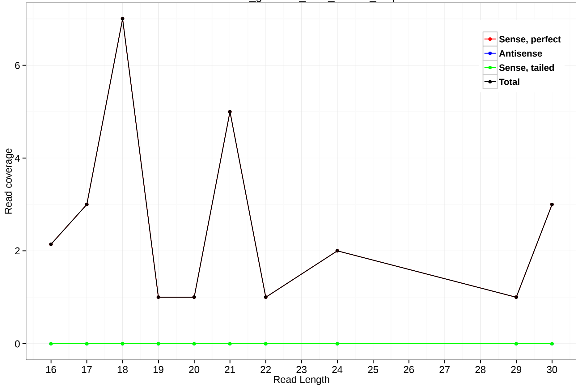
rheMac3_genscan_chr8_123.17_0.5p
