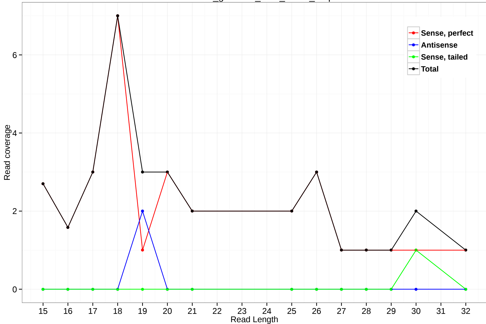
rheMac3_genscan_chr8_119.6_3.3p
