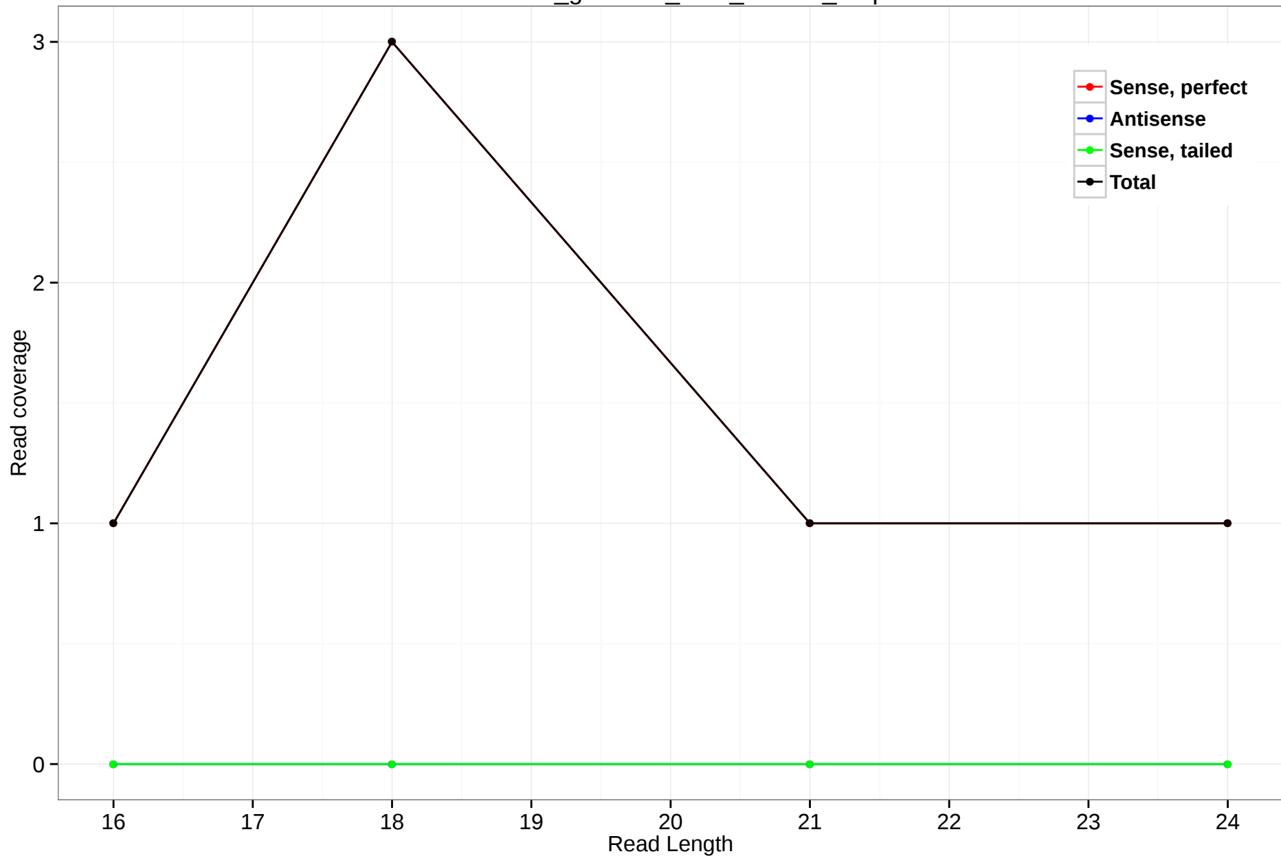
rheMac3_genscan_chr8_119.18_4.3p
