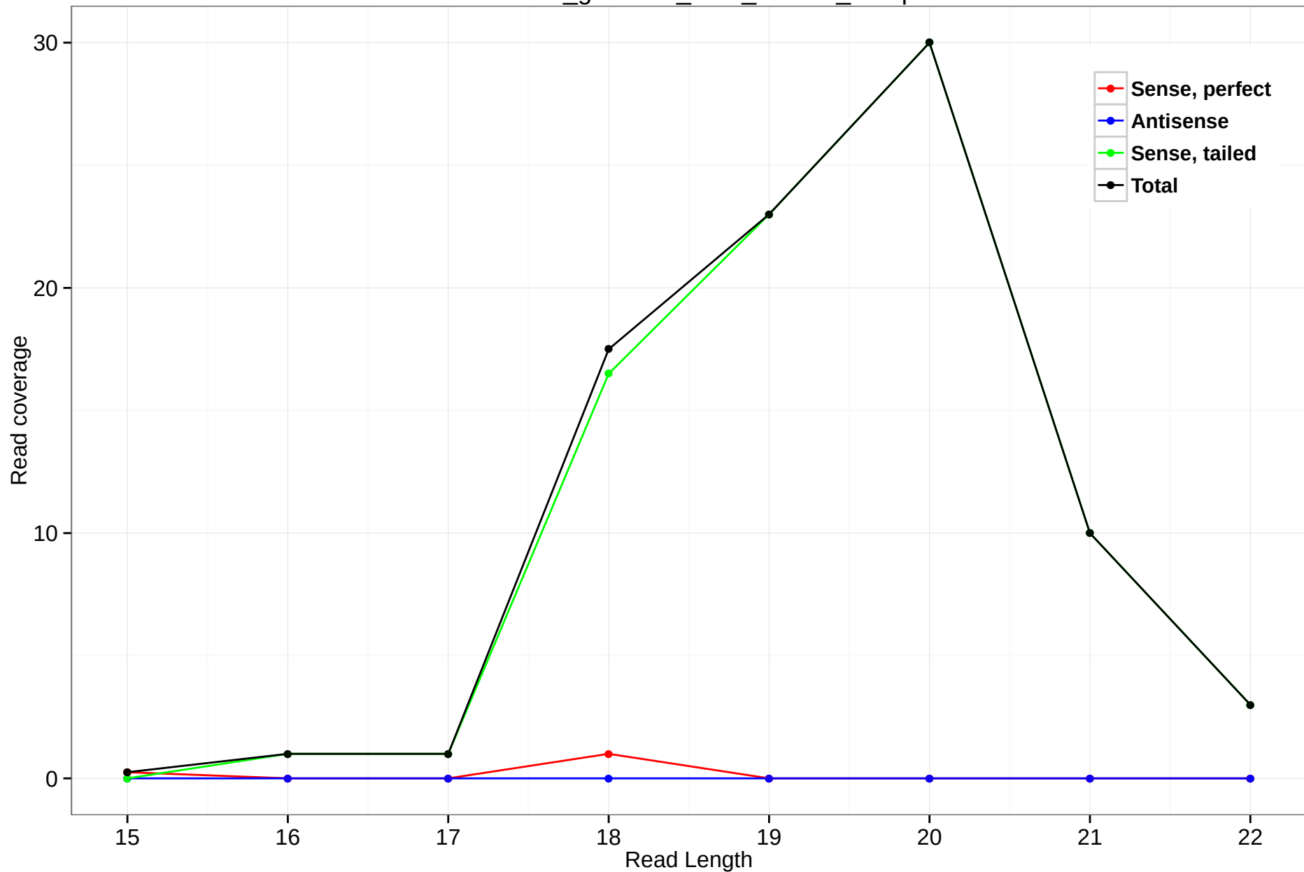
rheMac3_genscan_chr8_119.12_10.5p
