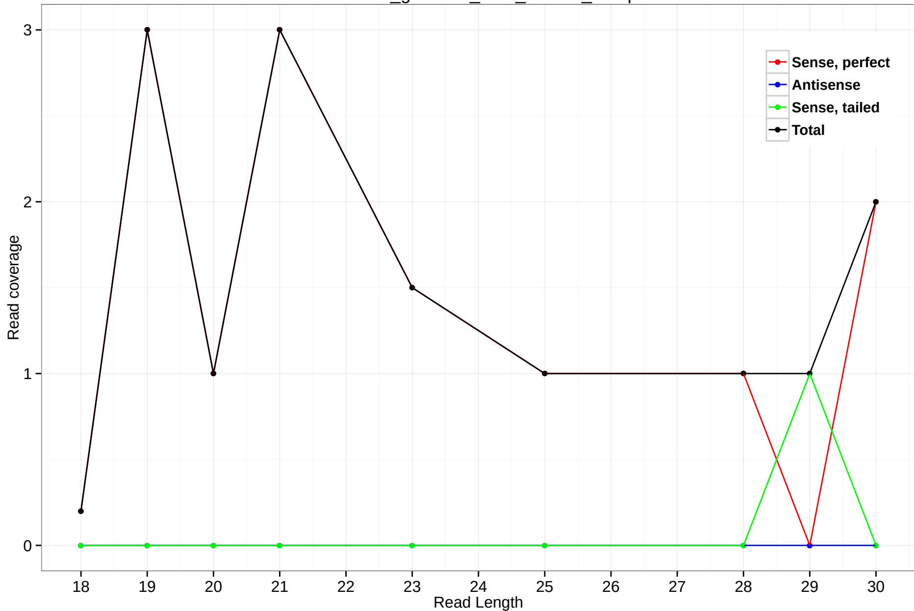
rheMac3_genscan_chr8_119.10_11.5p
