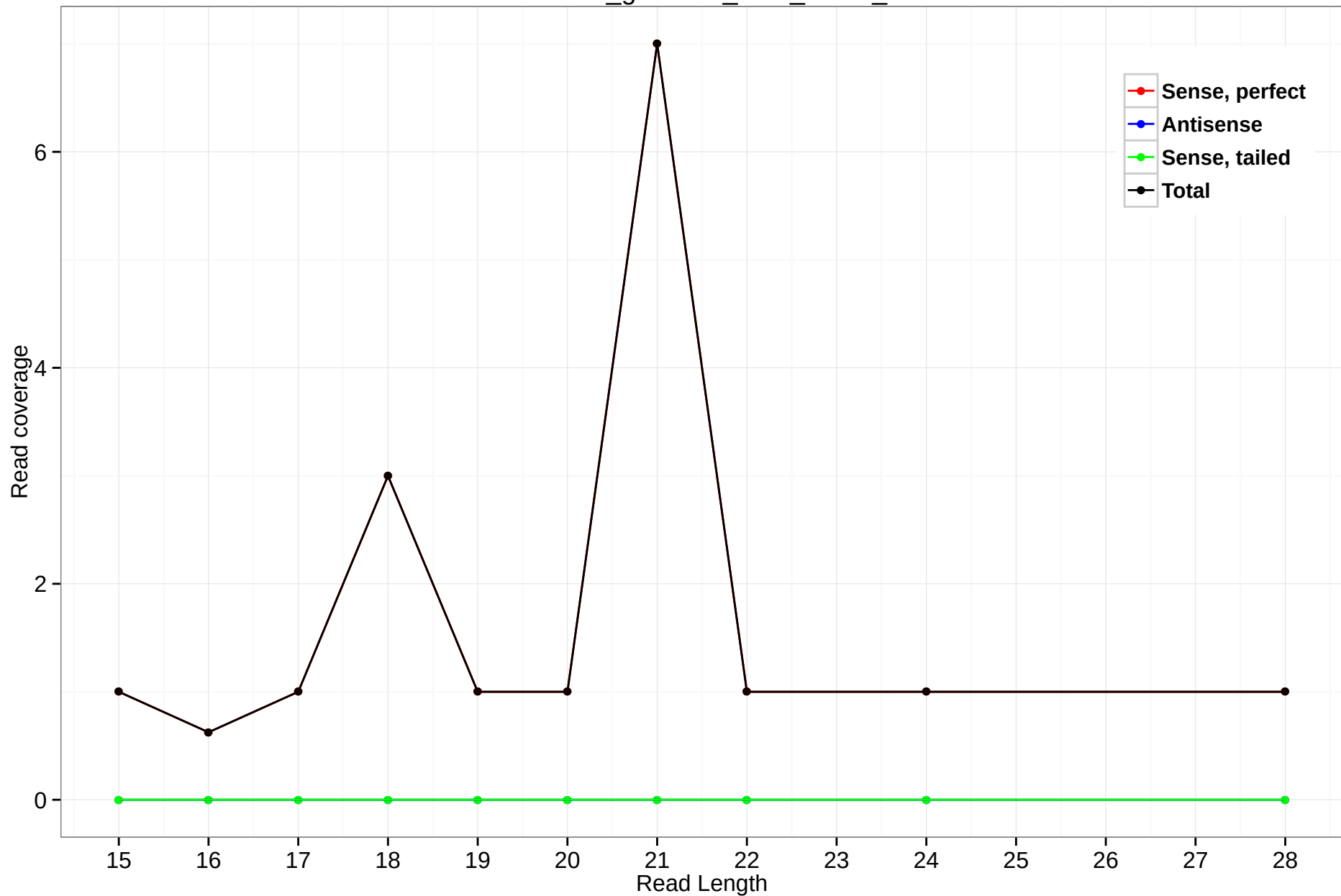
rheMac3_genscan_chr8_115.3_1
