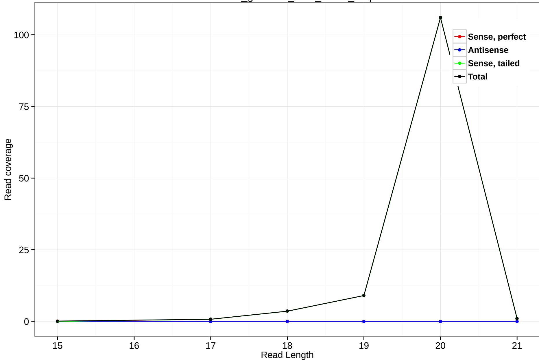
rheMac3_genscan_chr8_115.2_3.3p
