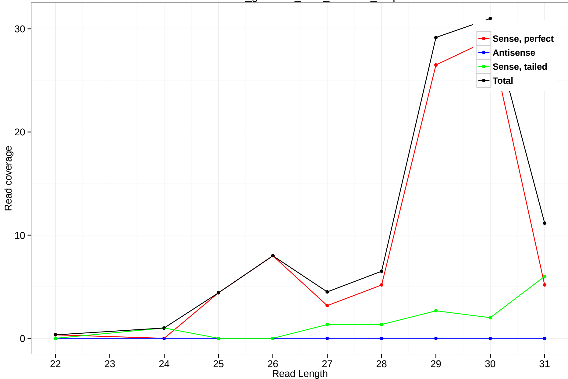
rheMac3_genscan_chr8_114.156_3.3p
