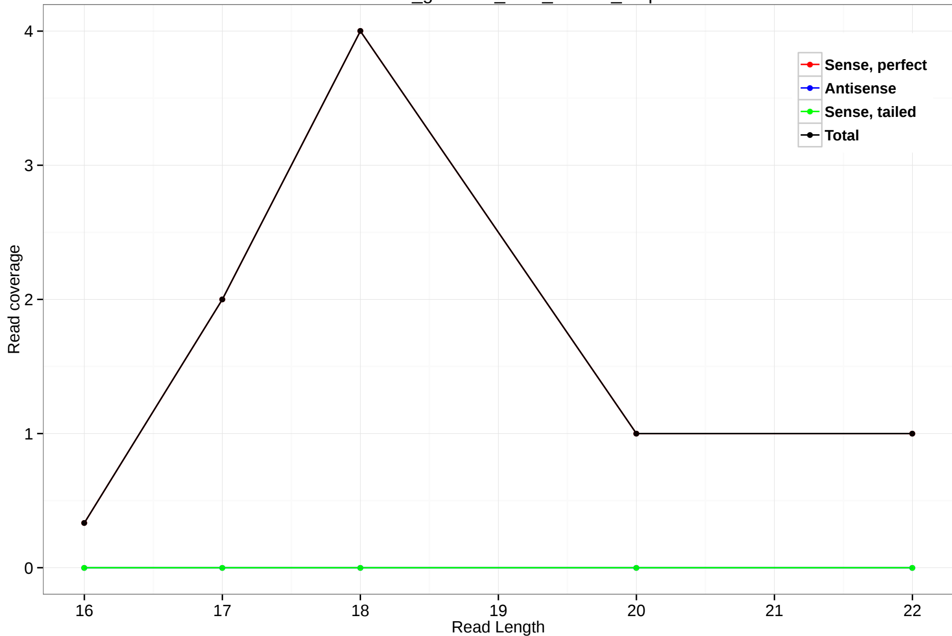
rheMac3_genscan_chr8_111.98_1.5p
