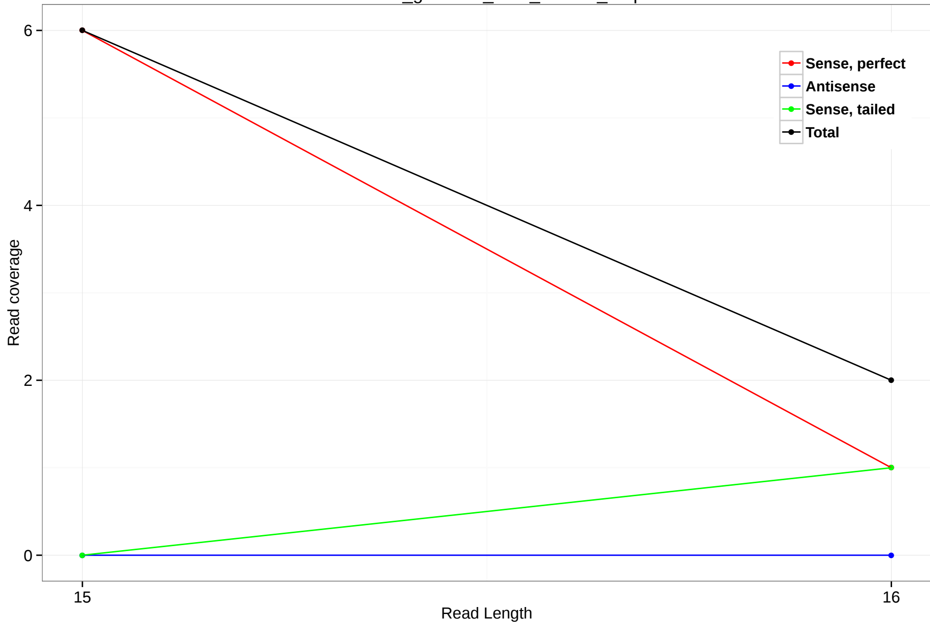
rheMac3_genscan_chr8_111.97_5.5p
