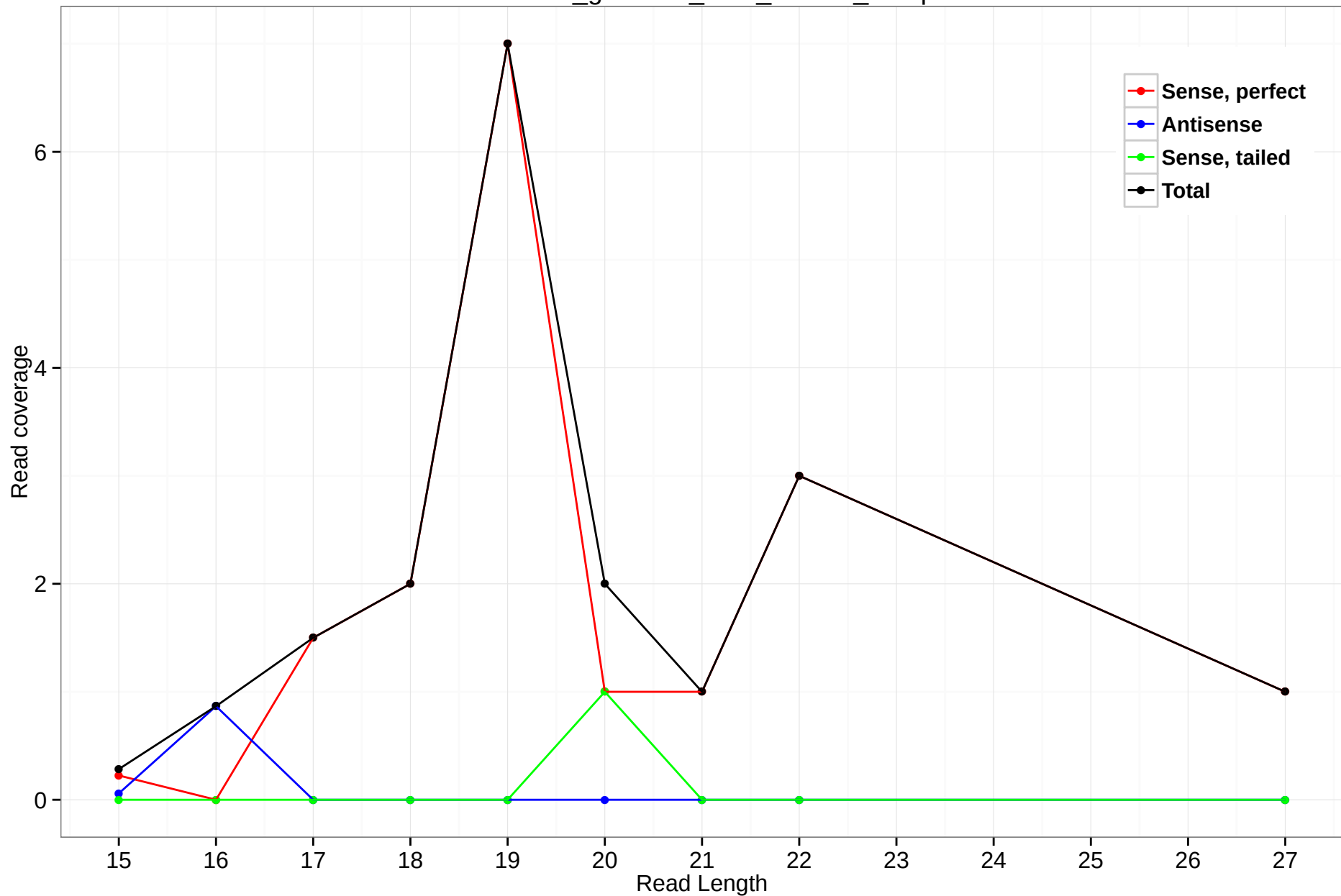
rheMac3_genscan_chr8_111.67_15.5p
