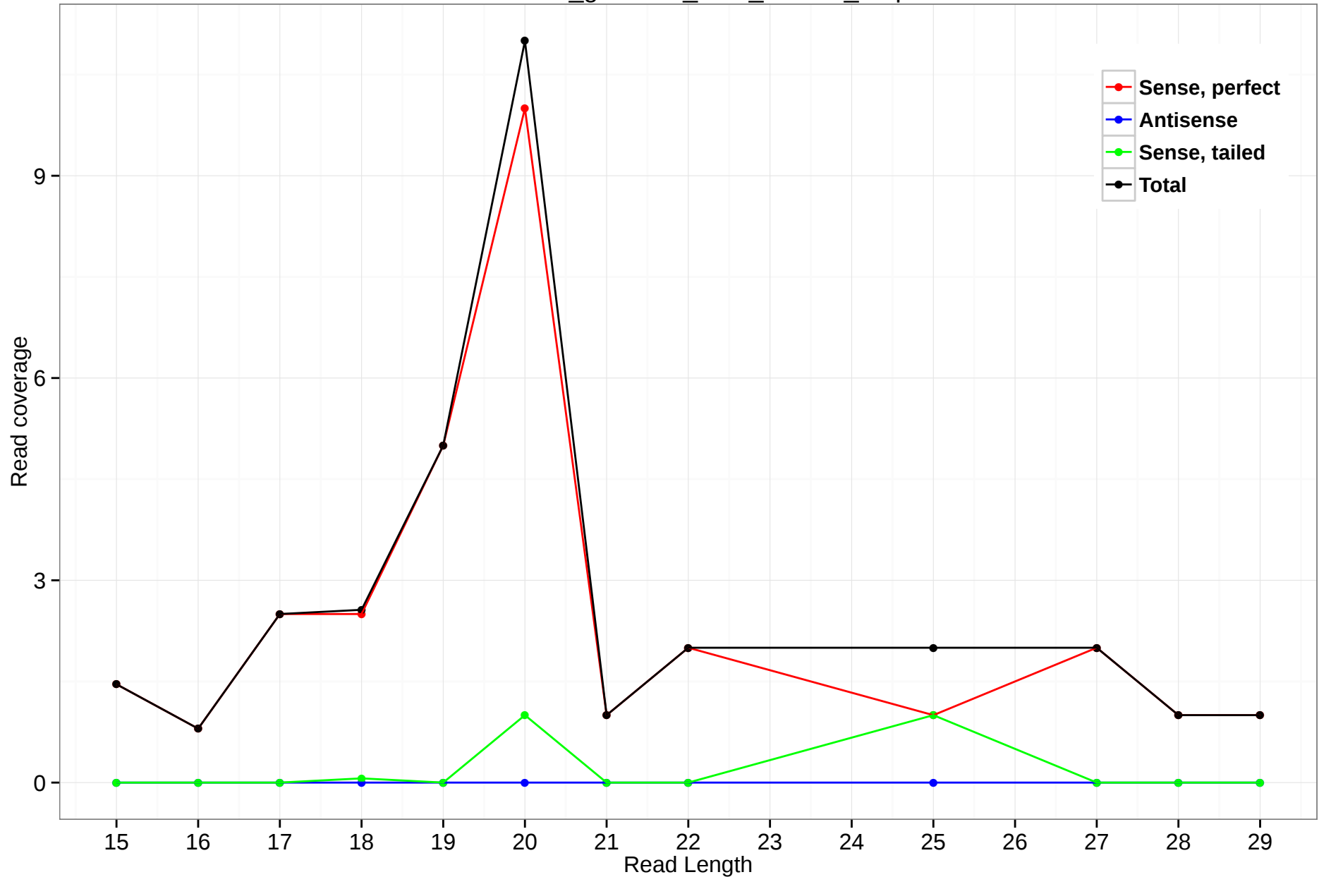
rheMac3_genscan_chr8_111.66_6.3p
