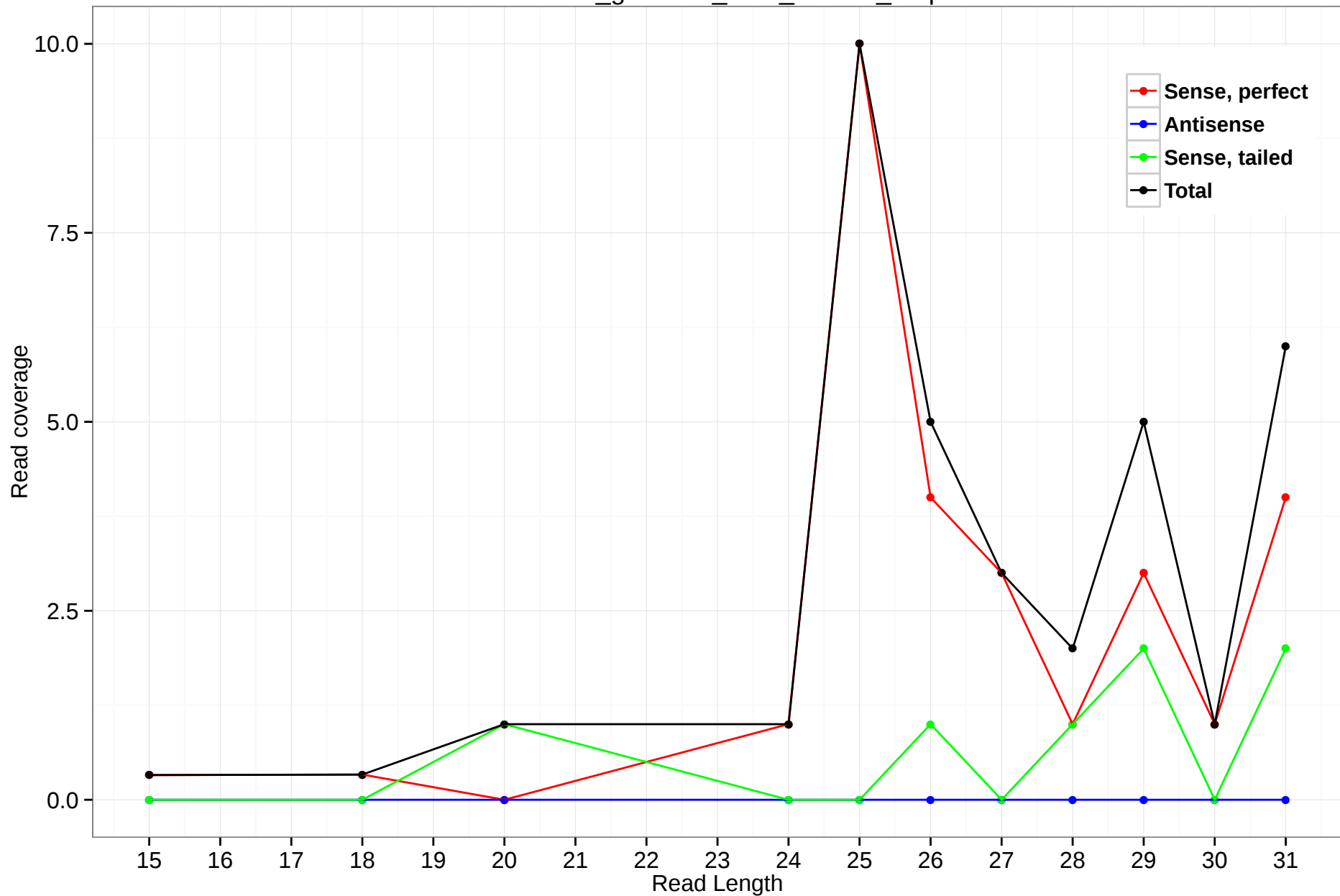
rheMac3_genscan_chr8_111.51_3.3p
