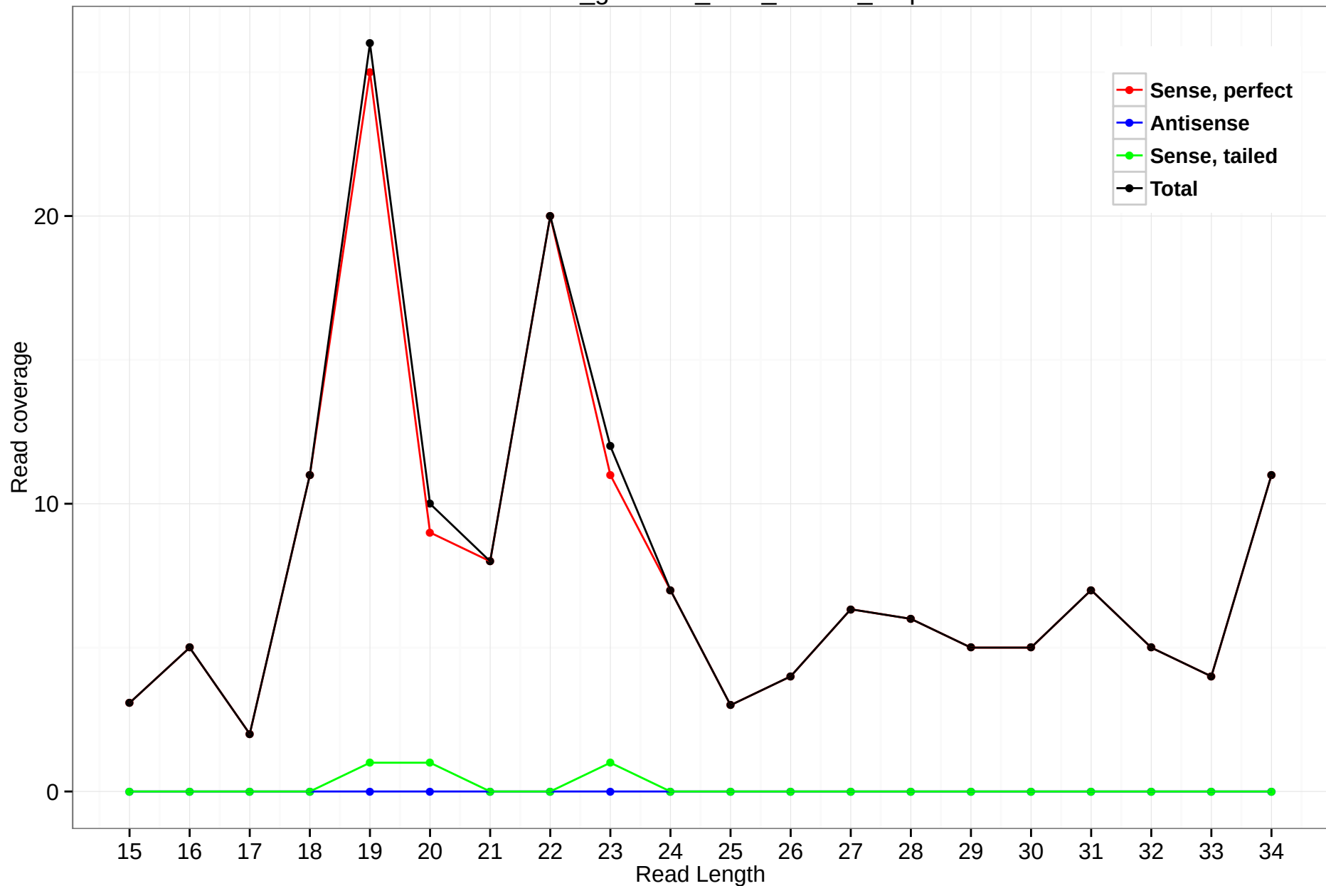
rheMac3_genscan_chr8_111.46_2.5p
