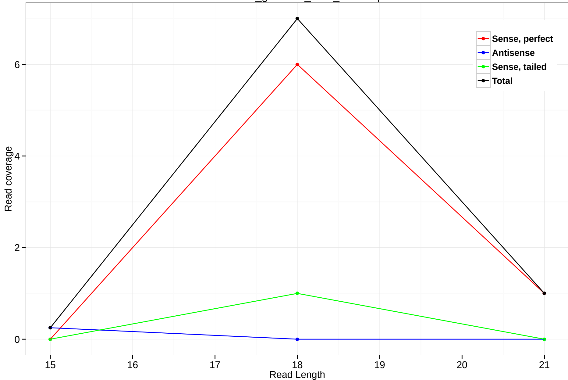
rheMac3_genscan_chr8_110.1.3p
