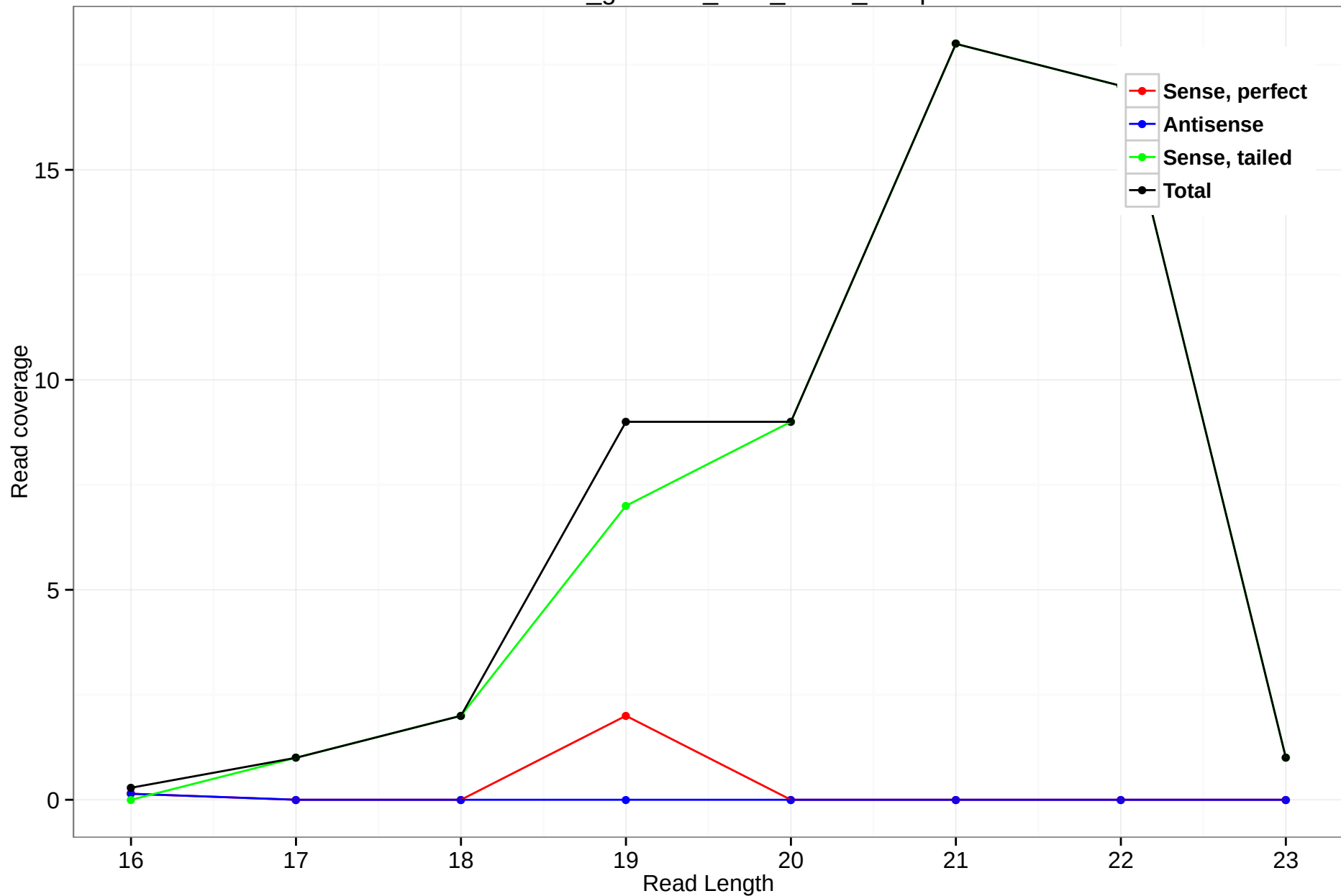
rheMac3_genscan_chr8_102.6_68.5p
