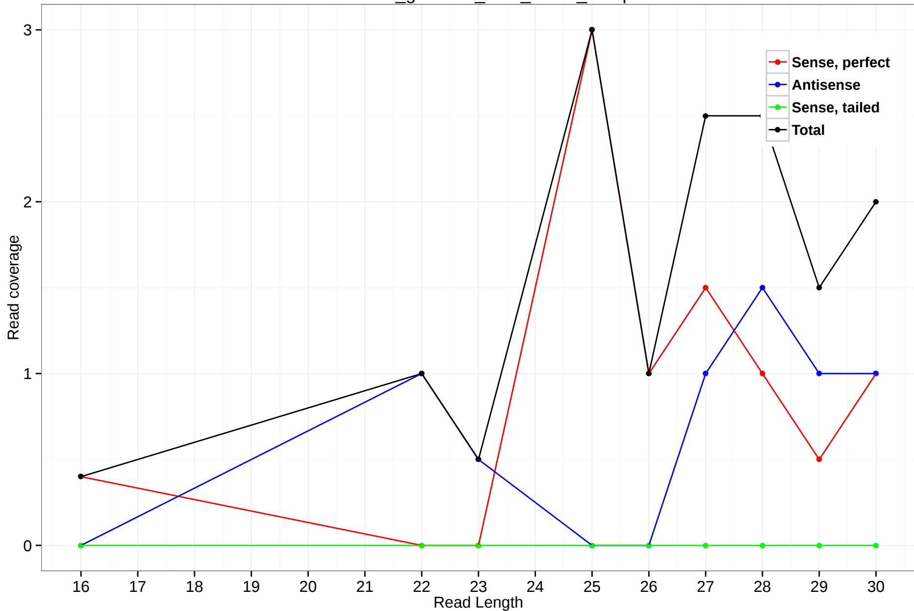
rheMac3_genscan_chr8_102.4_21.5p
