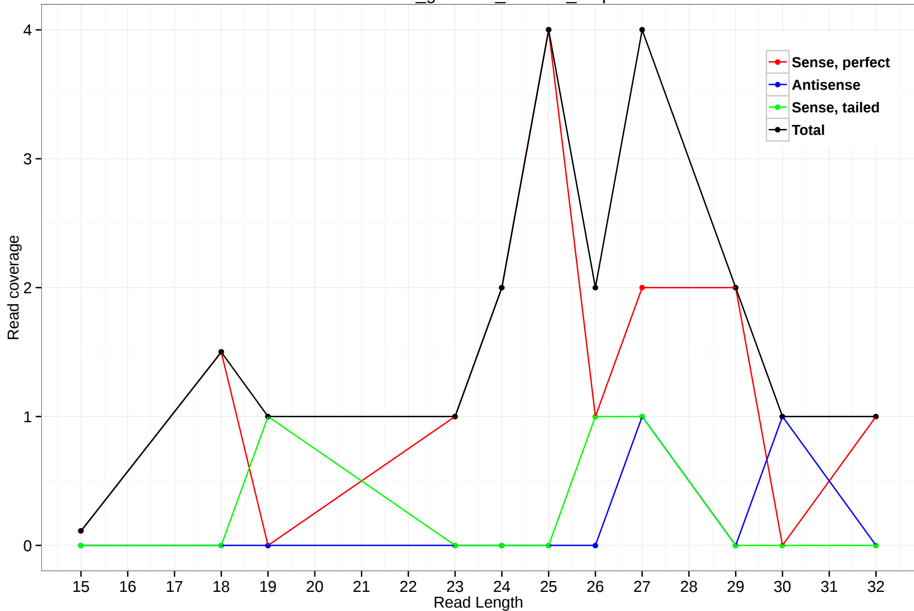
rheMac3_genscan_chr7.99_3.5p
