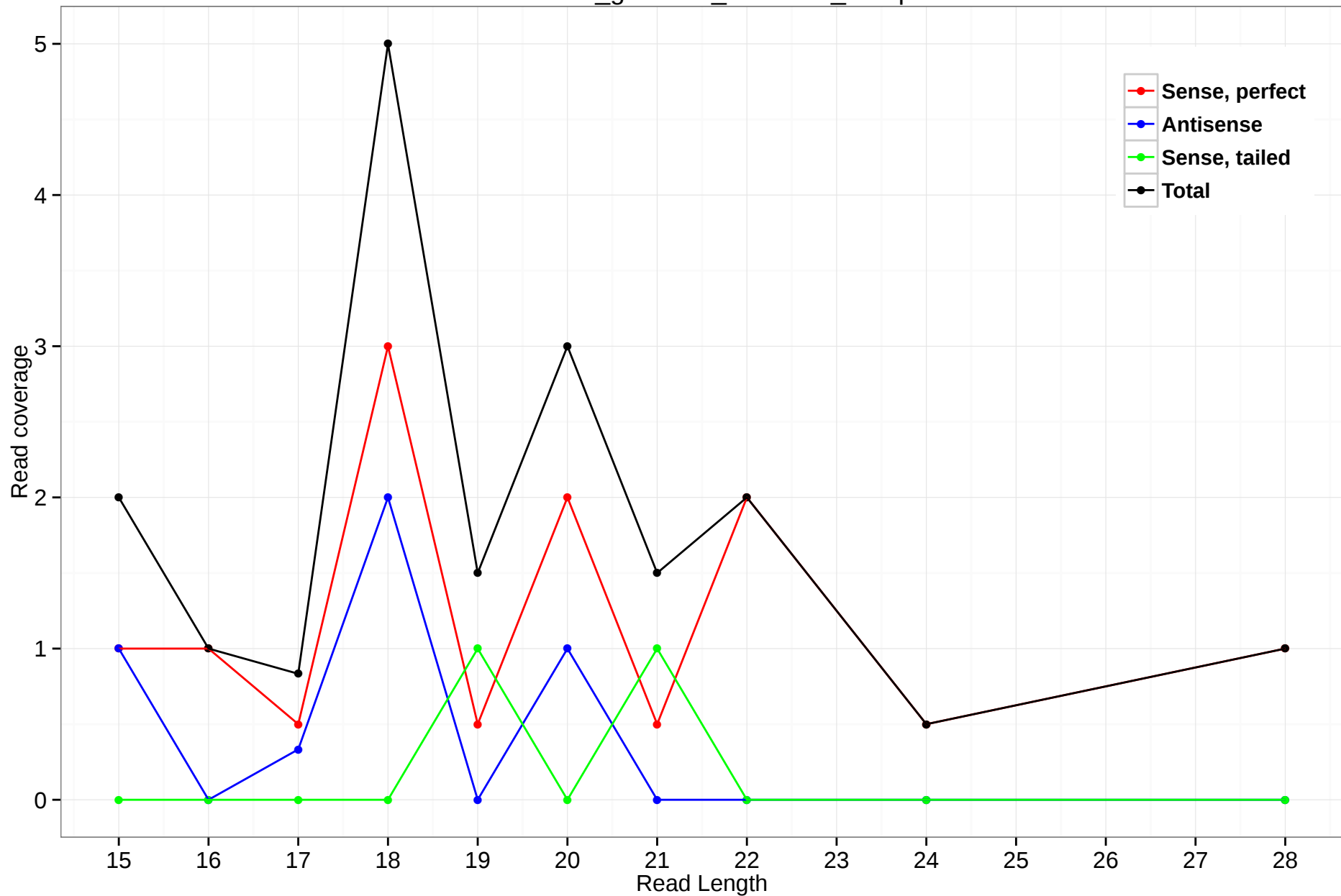
rheMac3_genscan_chr7.996_27.3p
