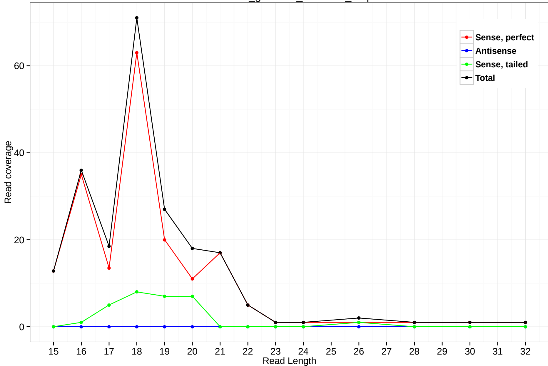
rheMac3_genscan_chr7.969_0.5p
