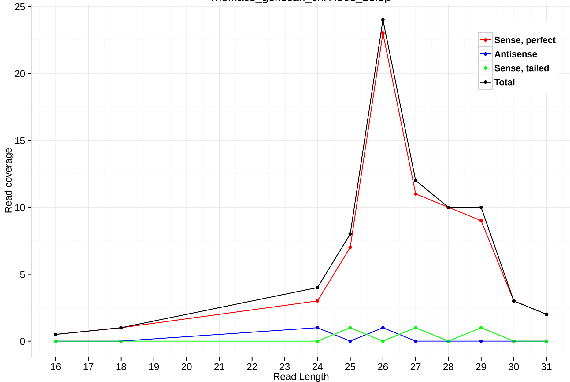
rheMac3_genscan_chr7.963_13.5p
