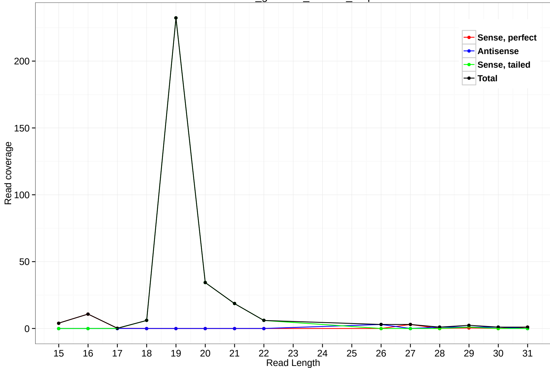
rheMac3_genscan_chr7.94_3.3p
